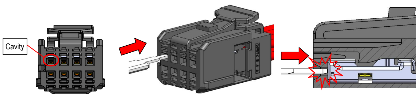
Fig. 42 Incorrect insertion of the terminal releasing jig
