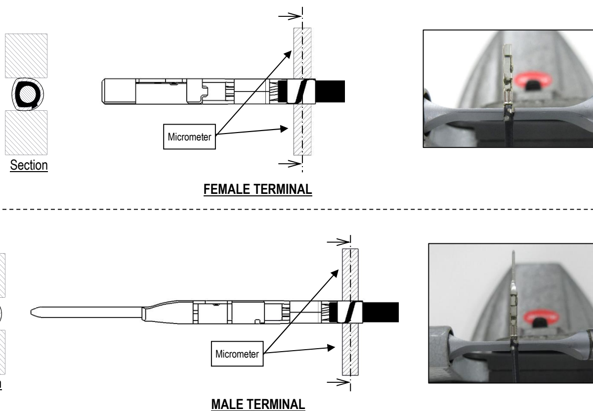
Fig 10. Insulation barrel crimp width measurement
