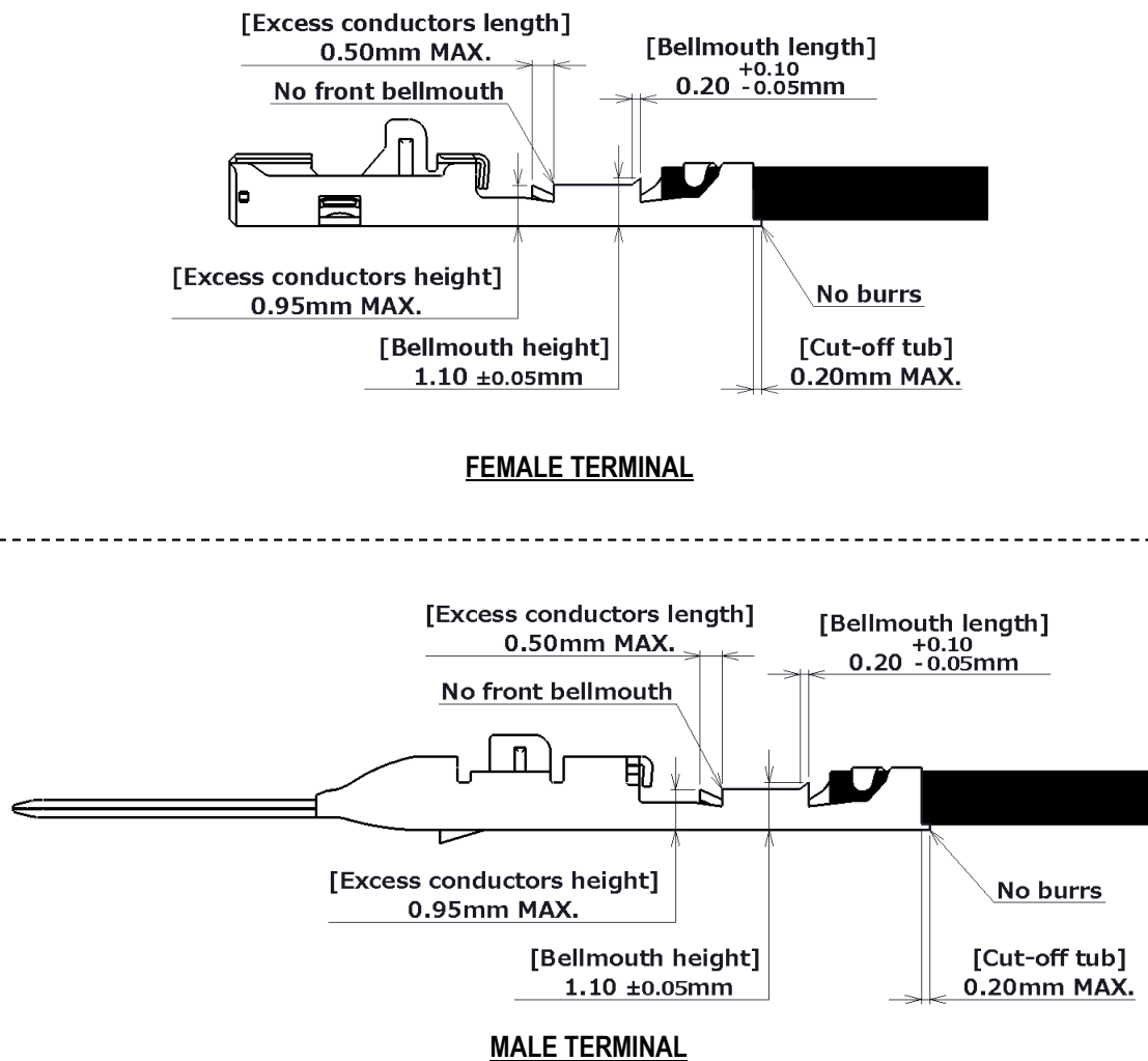
Fig.12 Bellmouth, excess conductors and cut-off tab
