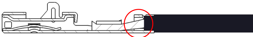
Fig.24 Strip too long
