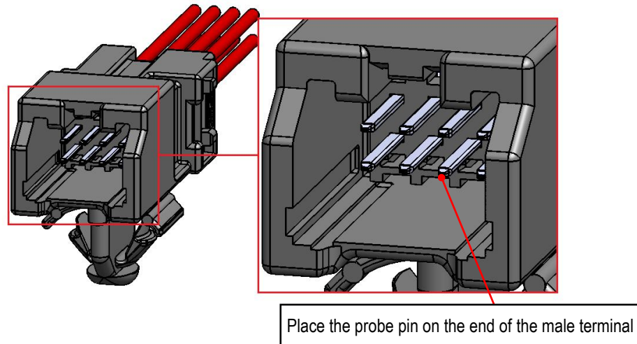
Fig.49 Conductivity test for male terminals (contacts)
