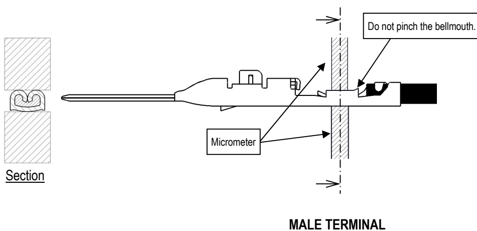
Fig 7. Wire barrel Crimp height measurement
