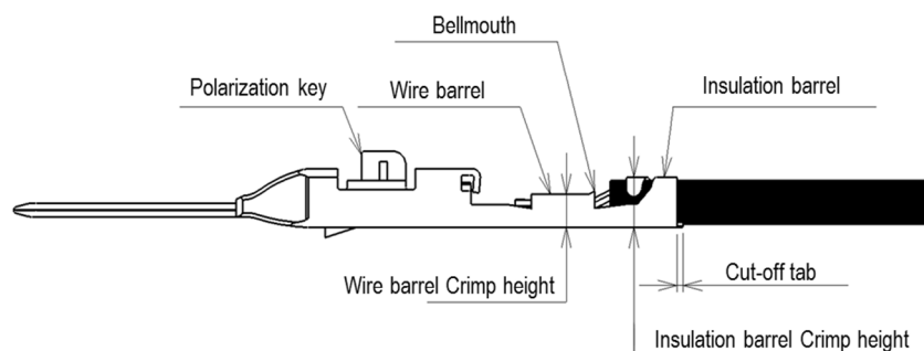
Fig.5 Male terminal part names
