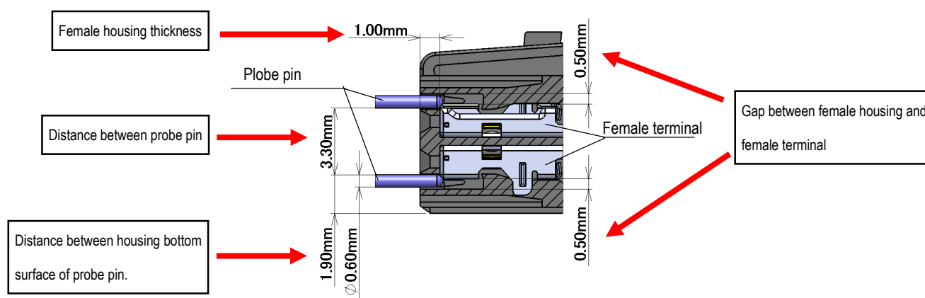
Fig.48 【Reference】Probe pin position on female connector
