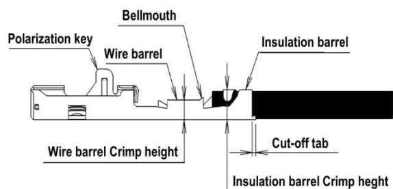
Fig.4 Female terminal part names
