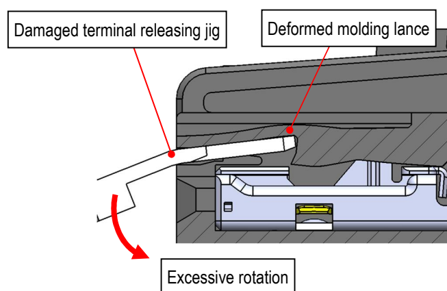
Fig.41 Deformed molding lance, Damaged releasing jig
