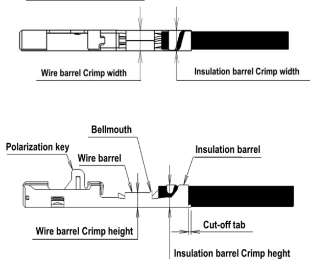
Fig.4 Female terminal part names
