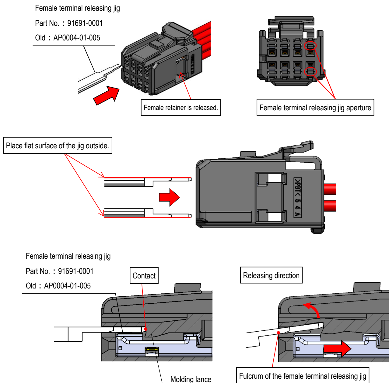
Fig.38 How to release the female terminal
