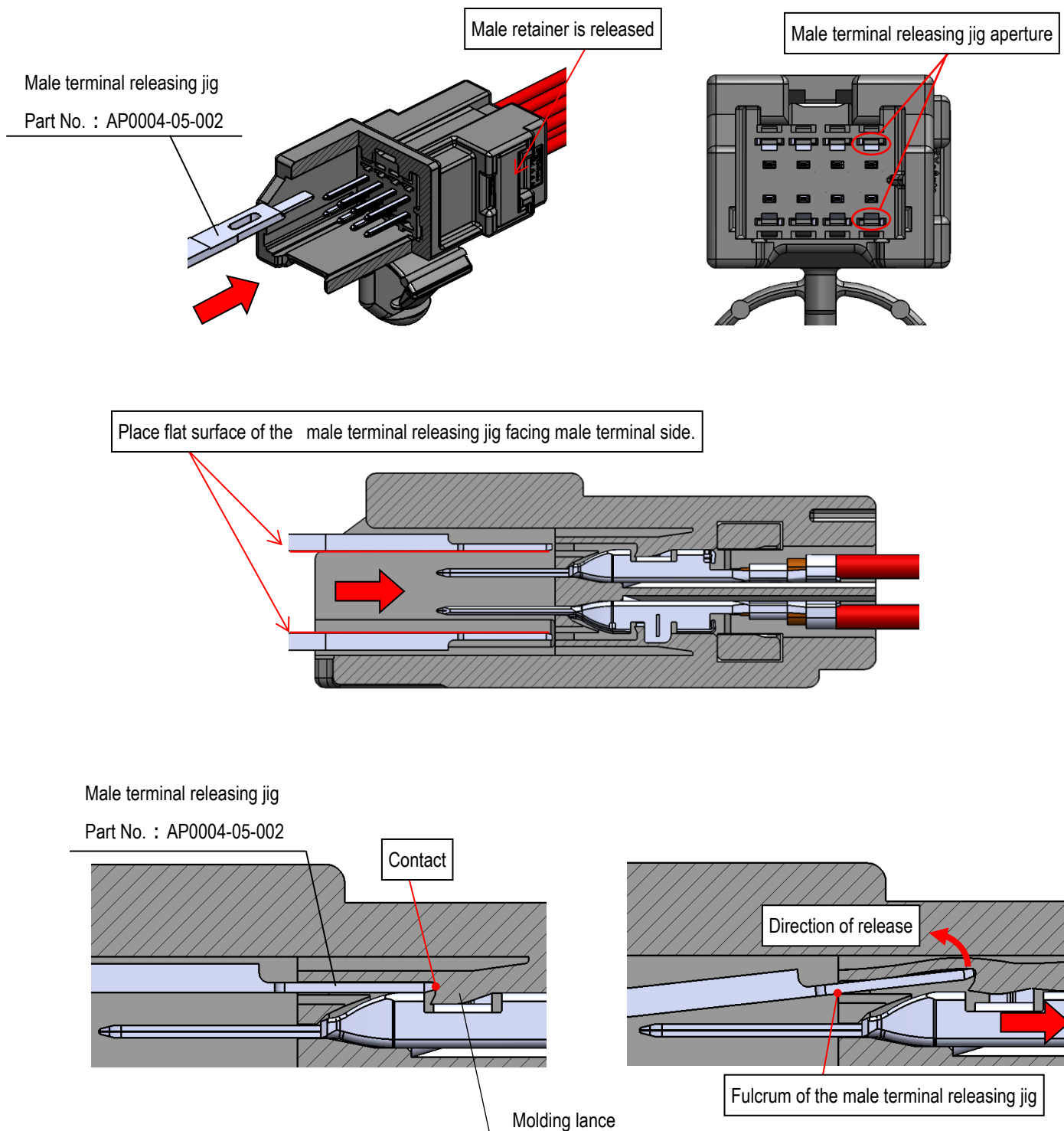
Fig.39 How to release the male terminal
