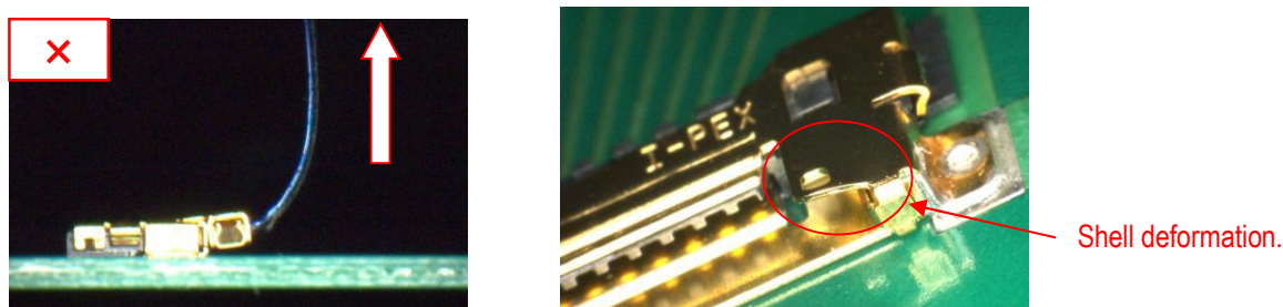
Vertical load.
