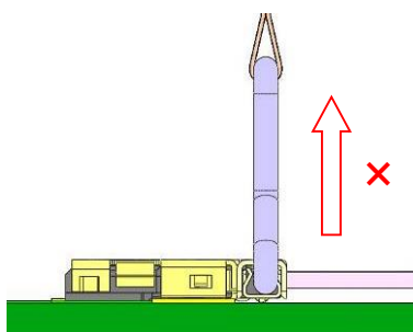
Vertical load.
