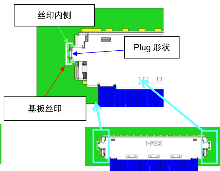
图.5 Without Lock cover
