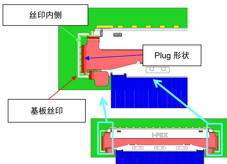
图.4 With Lock cover
