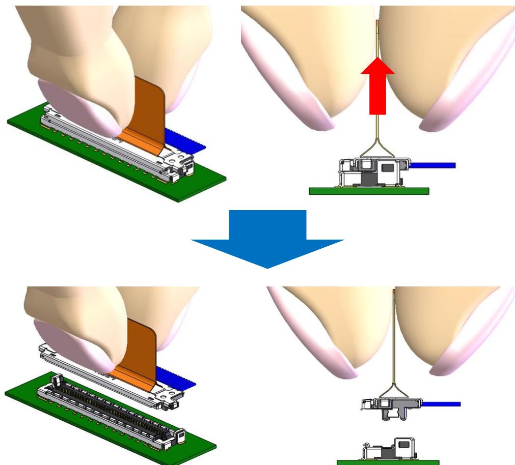
Fig.26 Unmating connectors by pulling PULL TAPE
