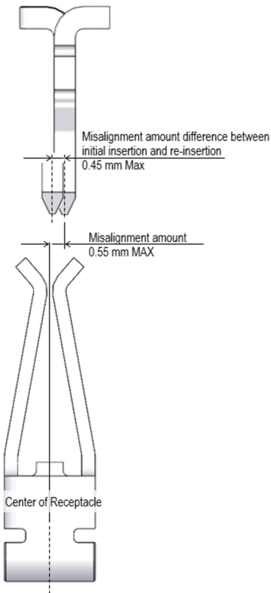
Fig.5 Condition of re-insertion
