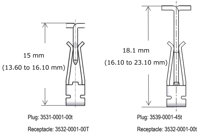
Fig.7 Mating Height
