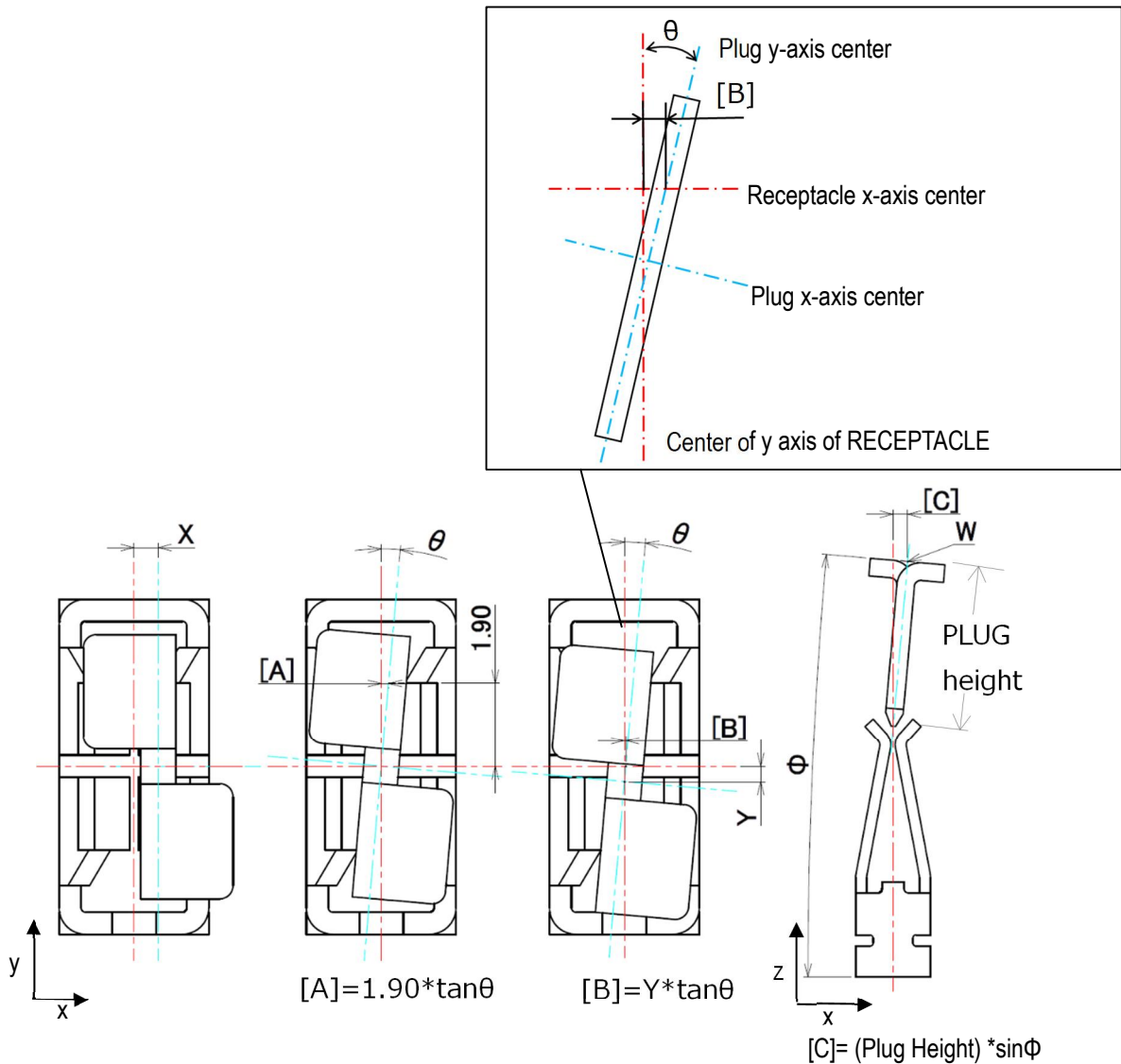
Fig.6 Misalignment component
