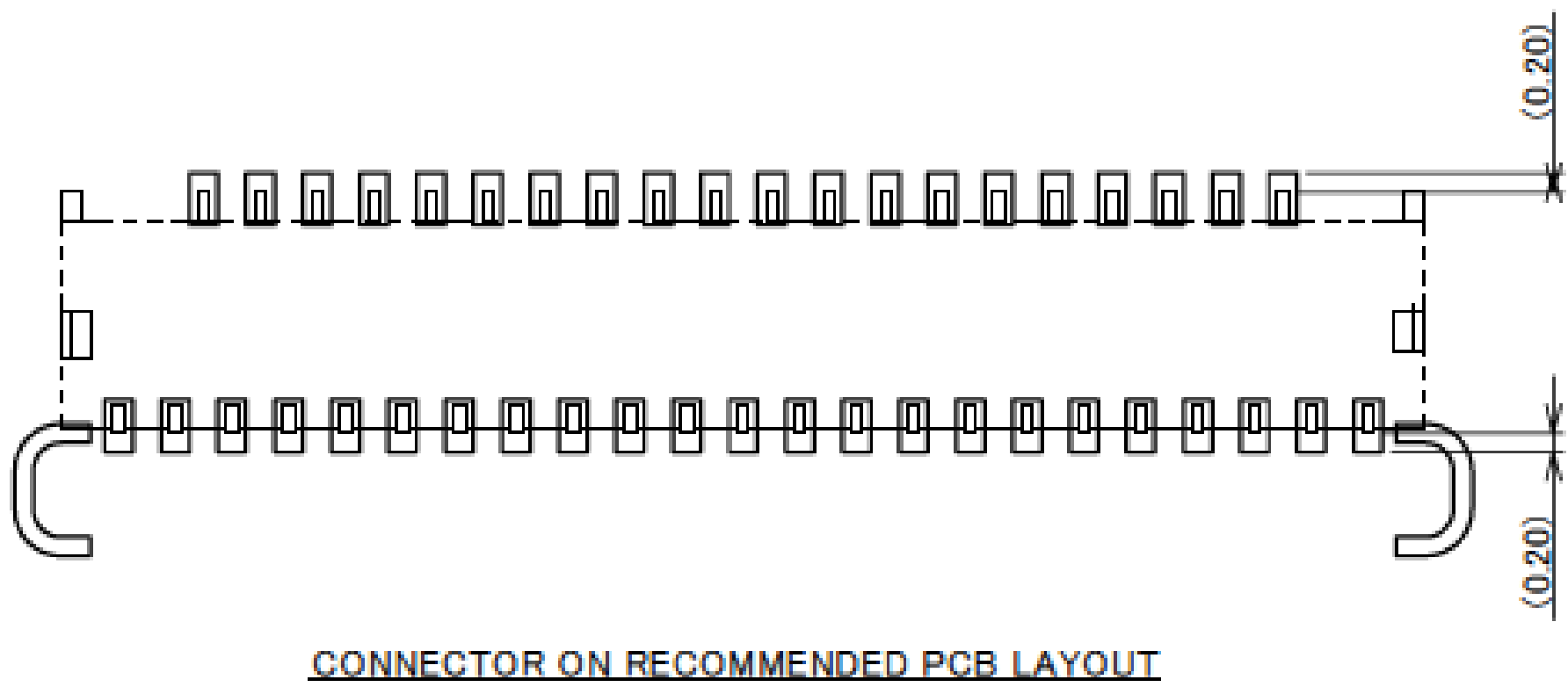
CONNECTOR ON RECOMMENDED PCB LAYOUT
