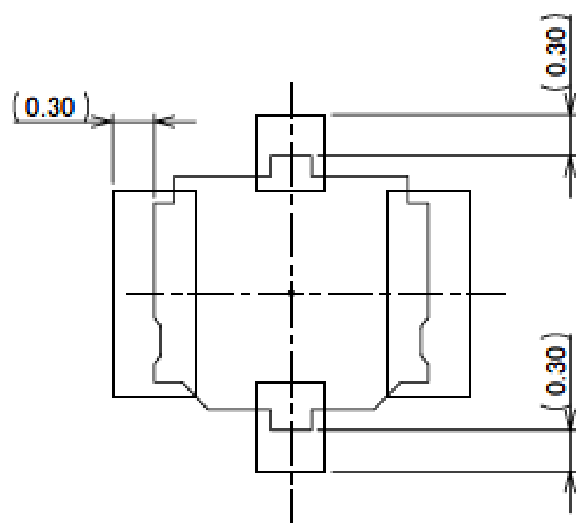
CONNECTOR ON RECOMMENDED FOOTPRINT PATTERN
