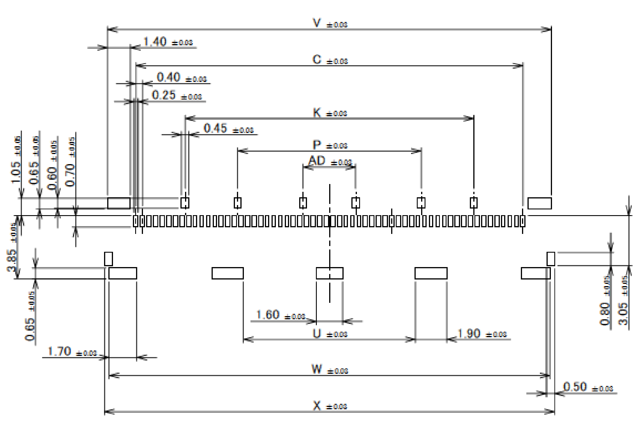
02 TYPE 60P RECOMMENDED METAL MASK LAYOUT (S = 5 : 1) ※ METAL MASK THICKNESS : t = 0.12
