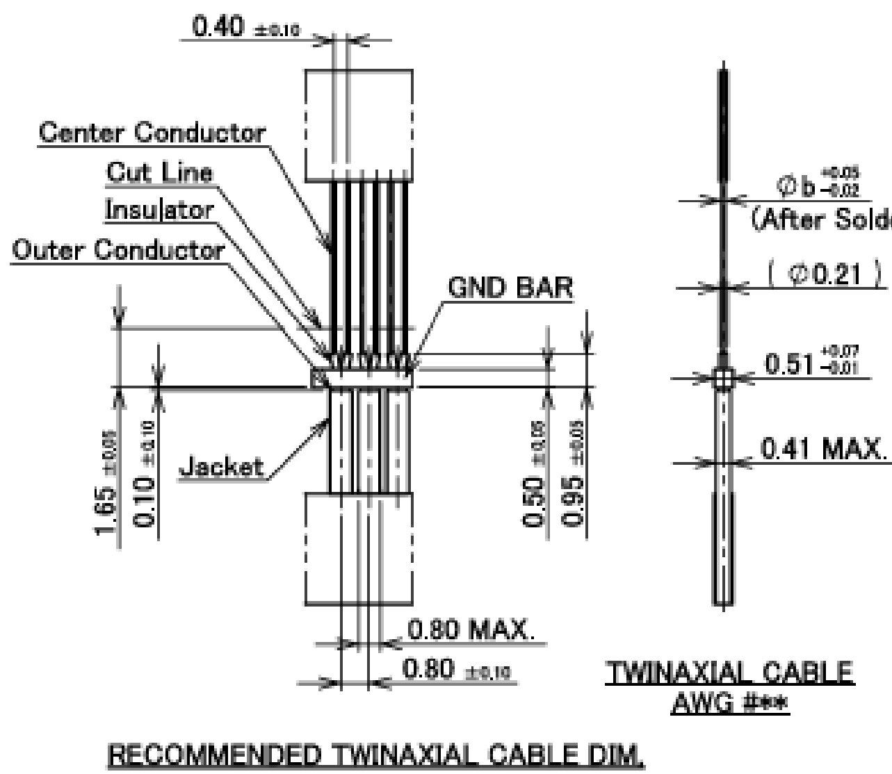
RECOMMENDED TWINAXIAL CABLE DIM.
