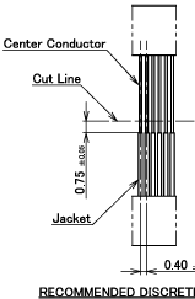
RECOMMENDED DISCRETE WIRE DIM.
