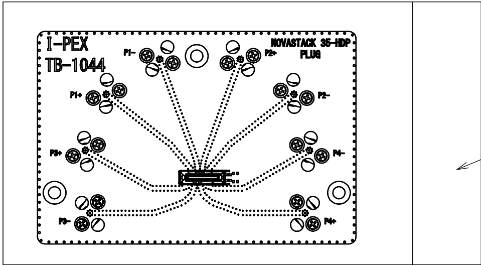
PLUG BOARD
