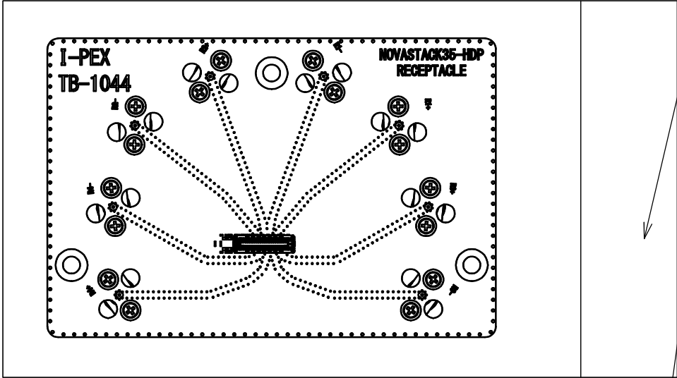
RECEPTACLE BOARD
