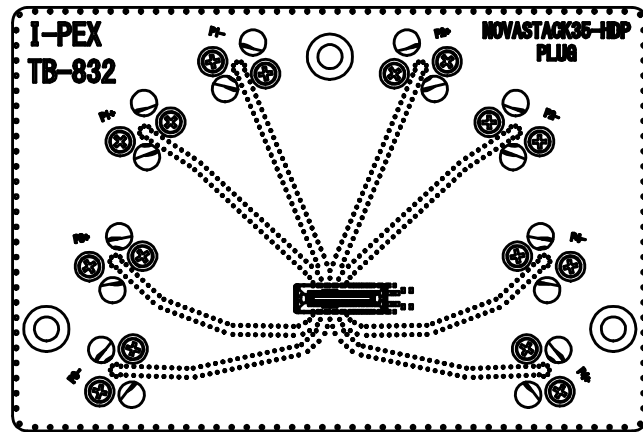
PLUG BOARD
