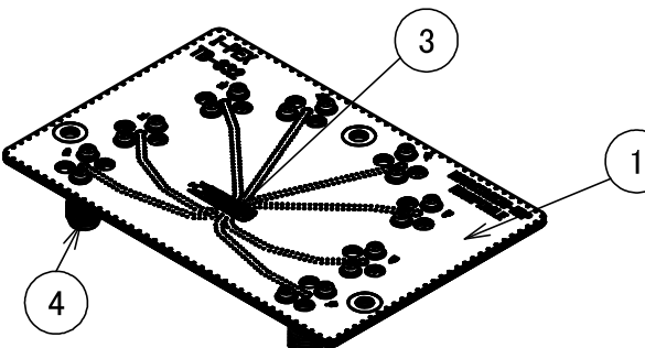
RECEPTACLE BOARD ASSEMBLY
