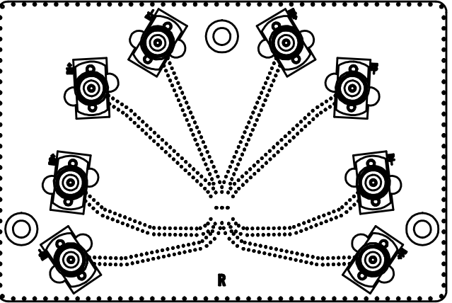
RECEPTACLE BOARD (JACK SIDE)
