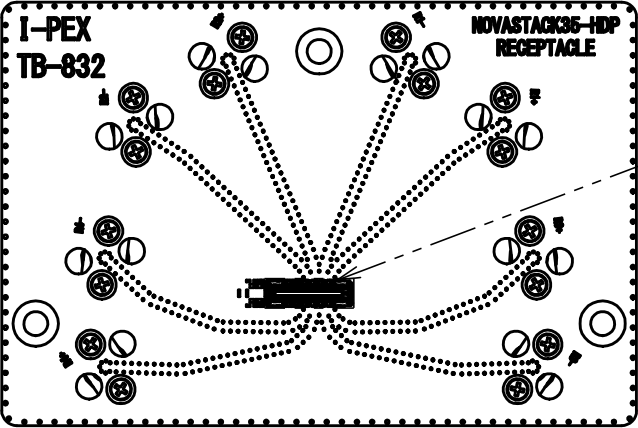
RECEPTACLE BOARD (CONNECTOR SIDE)
