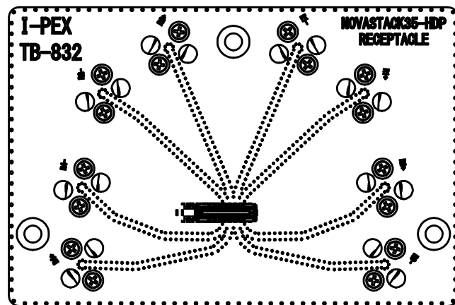
RECEPTACLE BOARD
