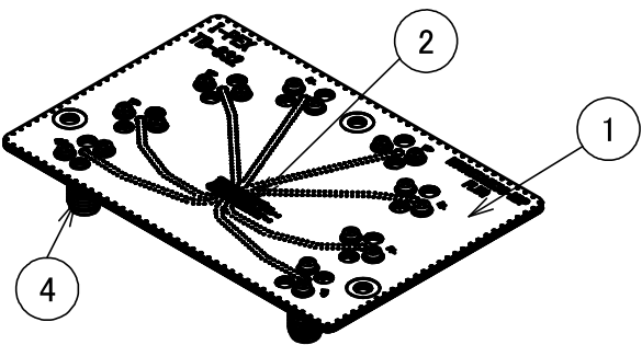
PLUG BOARD ASSEMBLY
