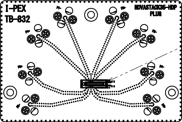
PLUG BOARD (CONNECTOR SIDE)
