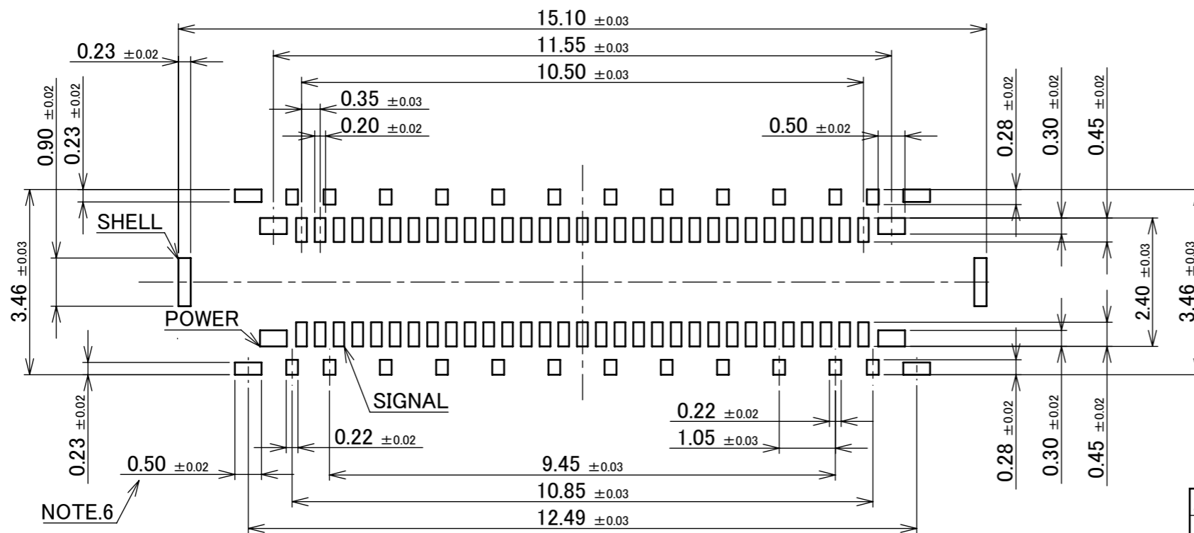
RECOMMENDED METAL MASK LAYOUT (62P)
