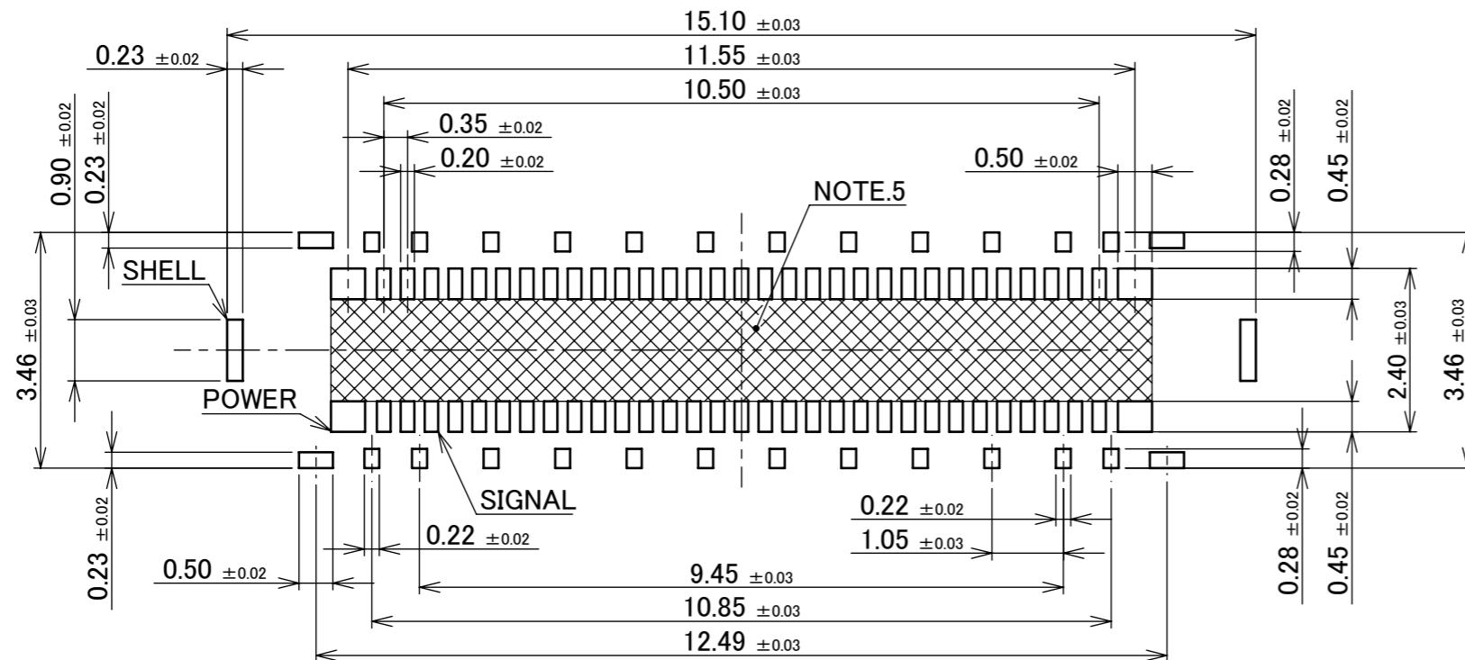
RECOMMENDED PATTERN LAYOUT (62P)
