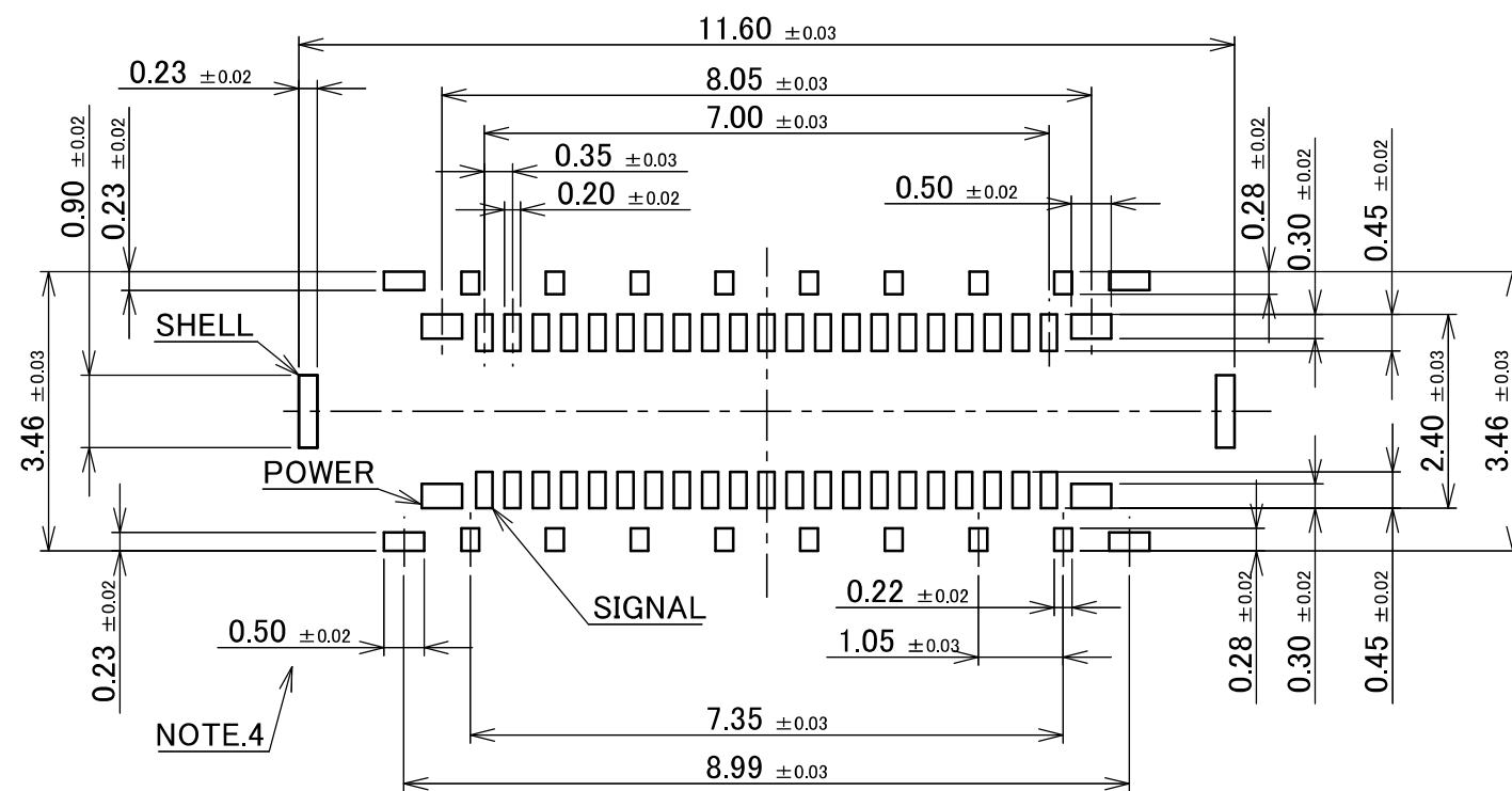
RECOMMENDED METAL MASK LAYOUT (42P) THICKNESS : t=0.10mm
