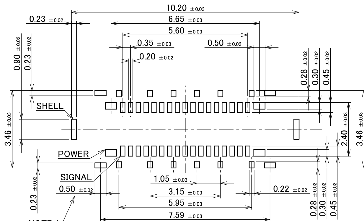
RECOMMENDED METAL MASK LAYOUT (34P) THICKNESS : t=0.10mm
