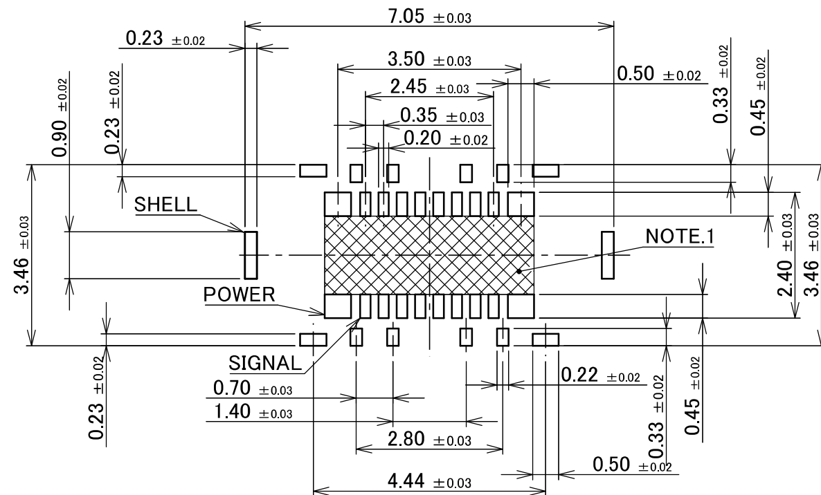
RECOMMENDED PATTREN LAYOUT (16P)
