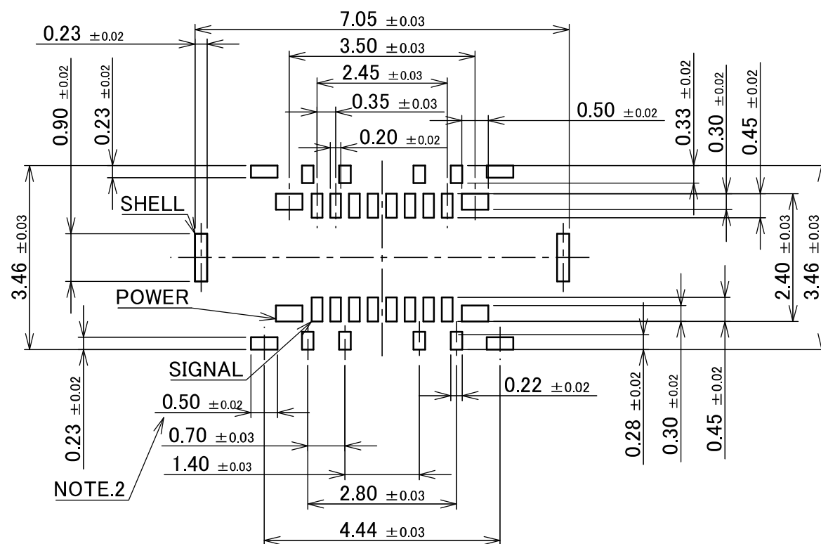
RECOMMENDED METAL MASK LAYOUT (16P) THICKNESS : t=0.10mm
