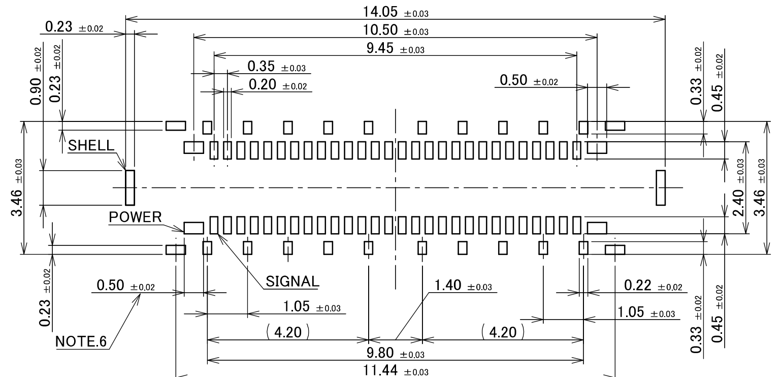
RECOMMENDED METAL MASK LAYOUT (56P) THICKNESS : t=0.10mm
