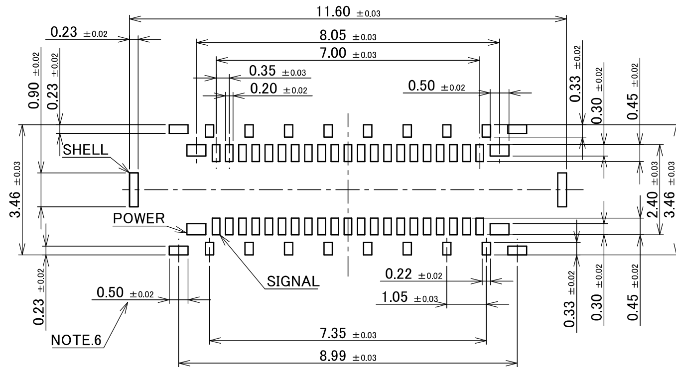
RECOMMENDED METAL MASK LAYOUT (42P) THICKNESS : t=0.10mm
