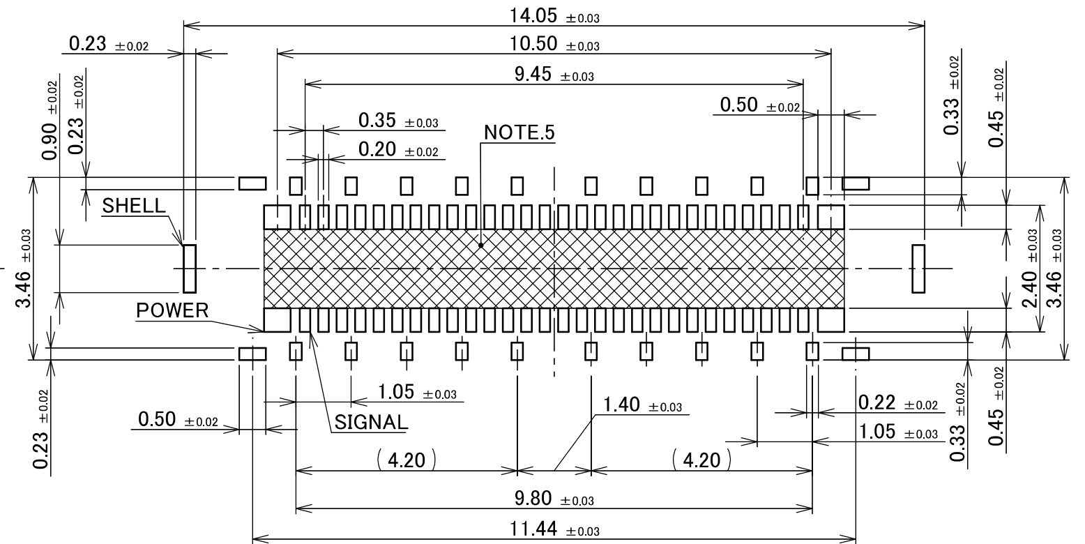
RECOMMENDED PATTERN LAYOUT (56P)
