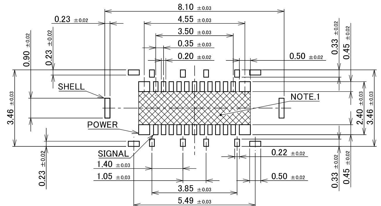
RECOMMENDED PATTREN LAYOUT (22P)
