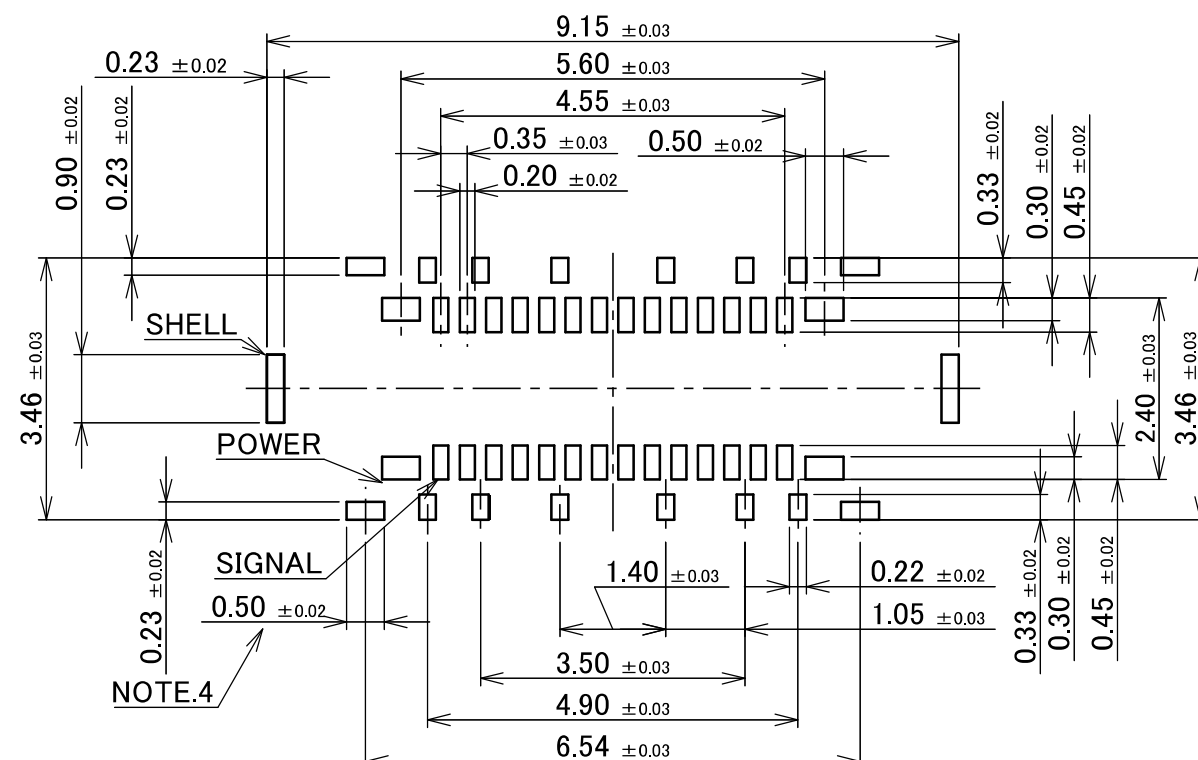
RECOMMENDED METAL MASK LAYOUT (28P) THICKNESS : t=0.10 mm
