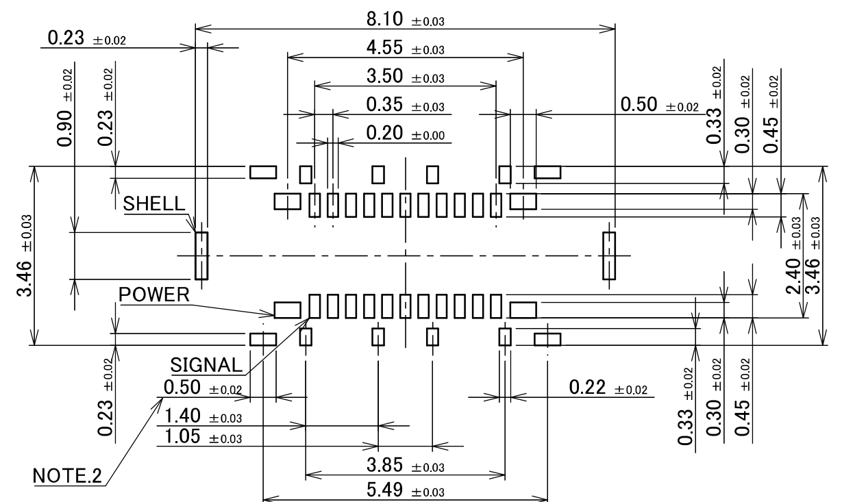
RECOMMENDED PATTREN LAYOUT (22P)
