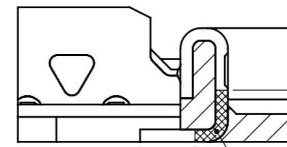
SECT. K-K (S=40:1)
