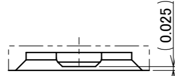
DETAIL M (S=40:1)
