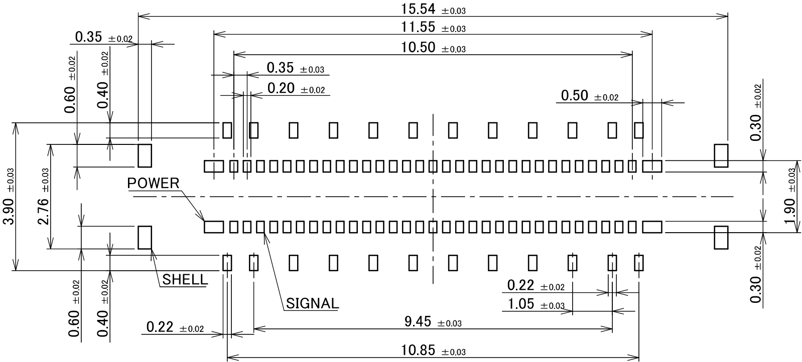
RECOMMENDED METAL MASK LAYOUT (62P) THICKNESS : t=0.10 mm
