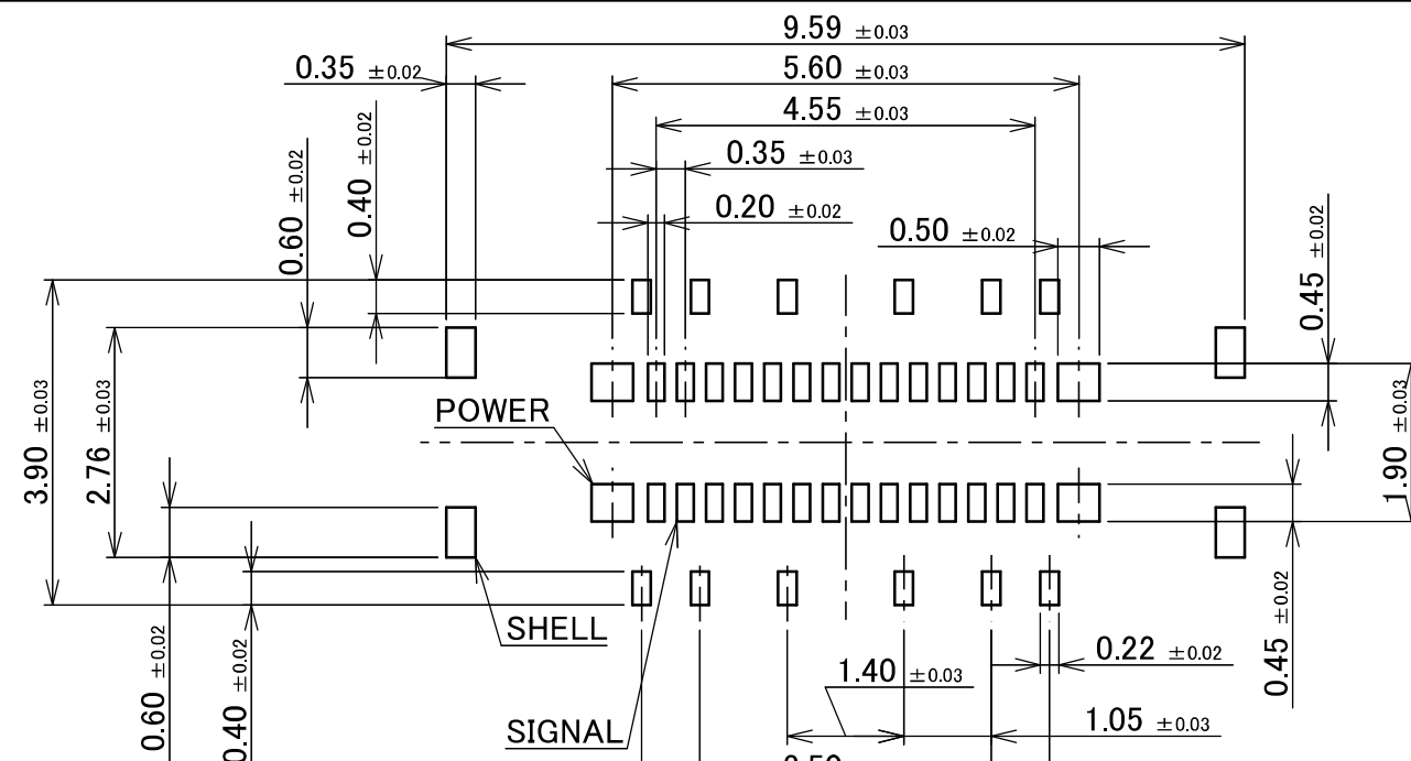
RECOMMENDED PATTERN LAYOUT (28P)
