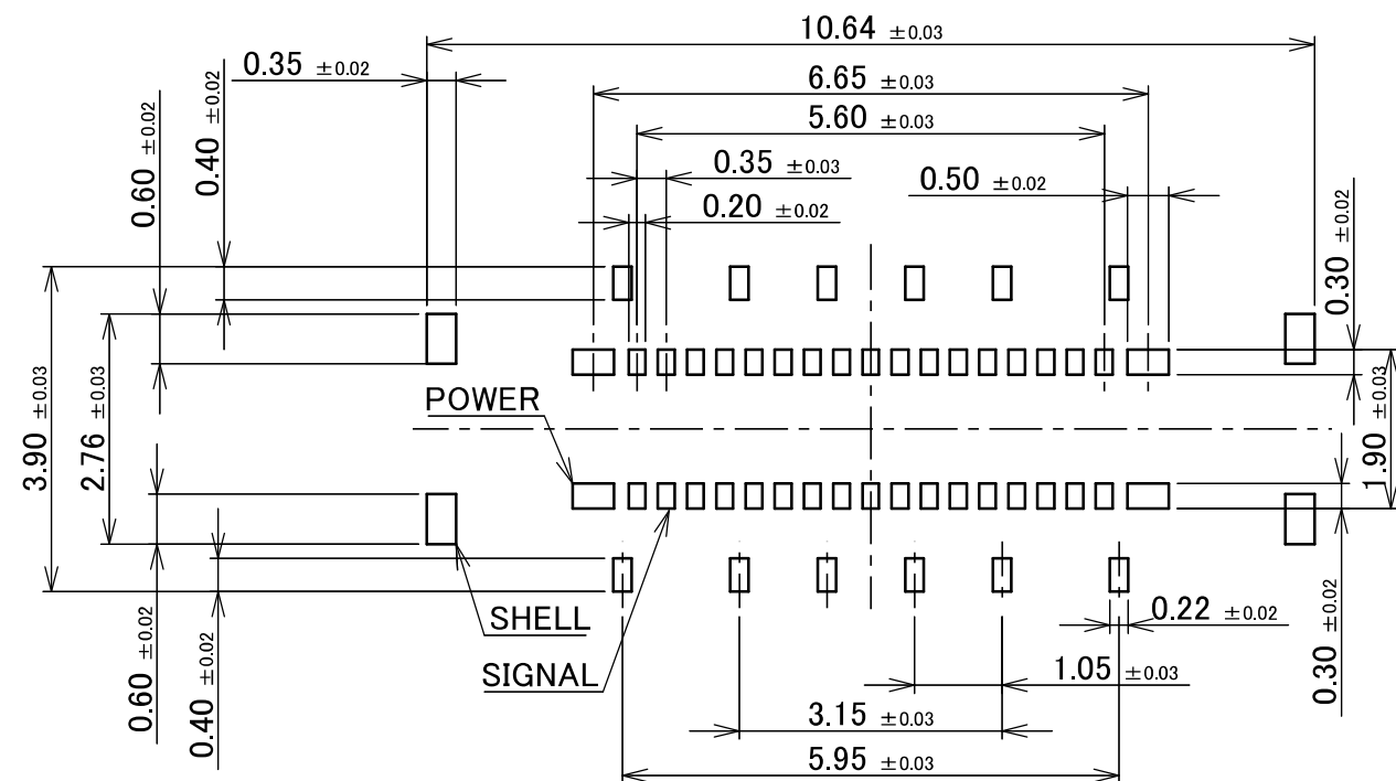
RECOMMENDED METAL MASK LAYOUT (34P) THICKNESS : t=0.10 mm
