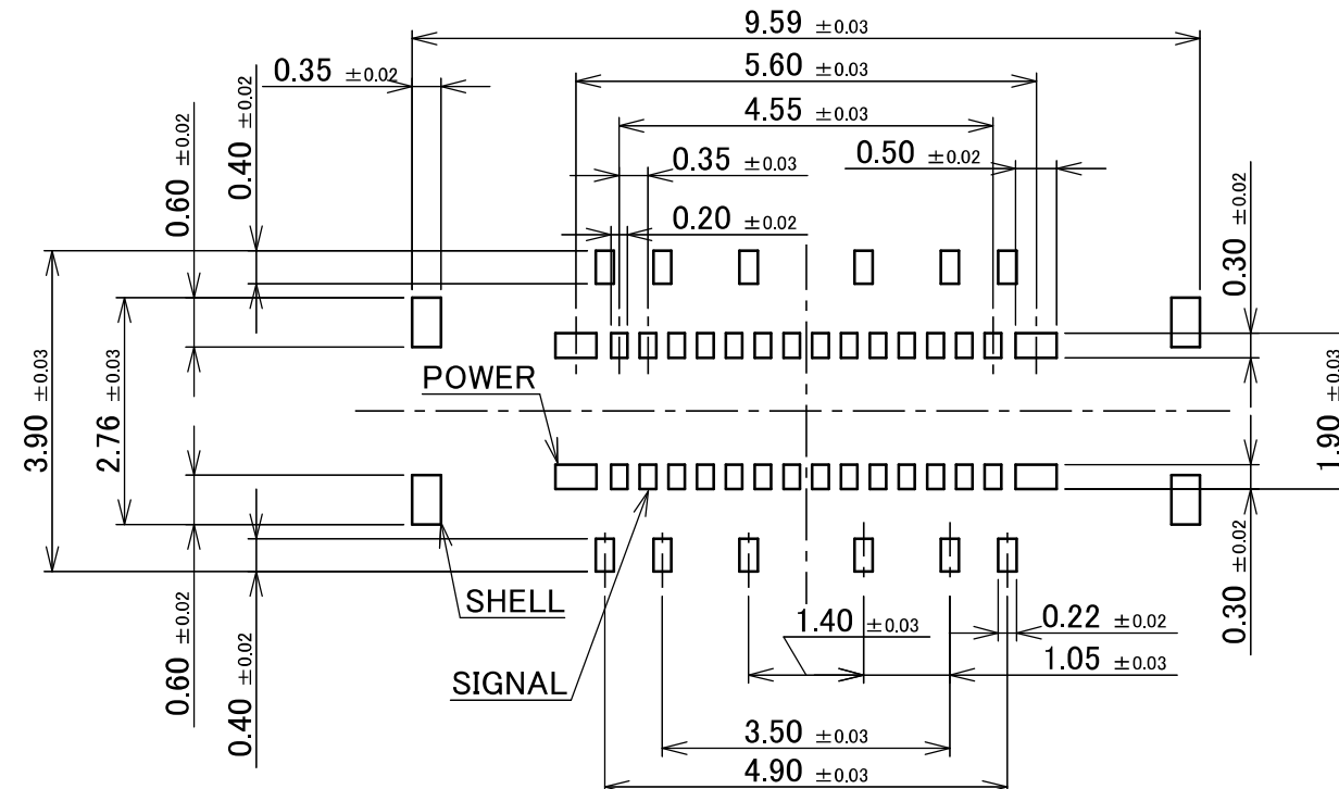
RECOMMENDED METAL MASK LAYOUT (28P) THICKNESS : t=0.10 mm
