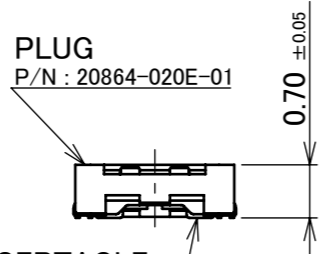
RECEPTACLE P/N: 20865-020E-03 MATING CONDITION
