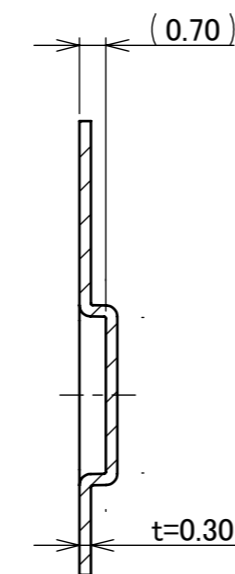
SECT. X-X (S=5:1)
