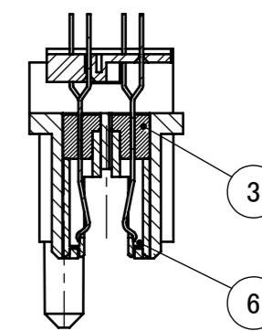
SECT. A-A
