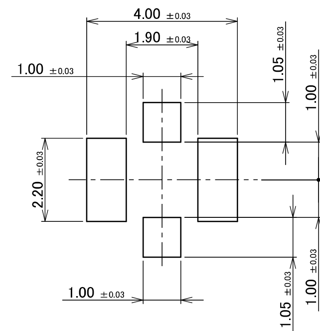
MASK THICKNESS: t = 0.12
