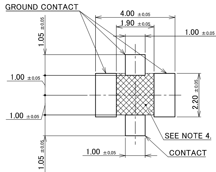
RECOMMENDED FOOTPRINT PATTERN
