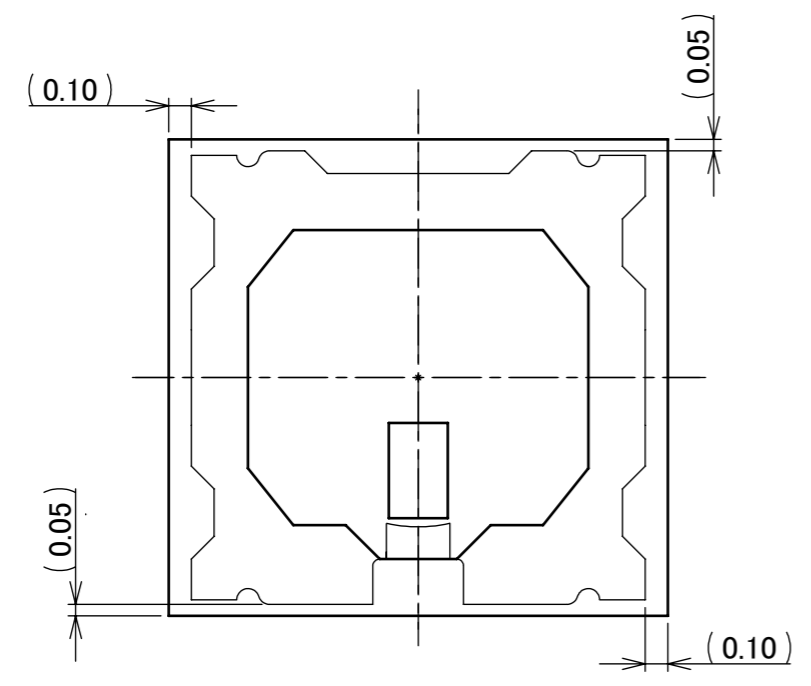
CONNECTOR ON RECOMMENDED FOOTPRINT PATTERN
