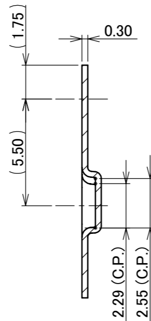
SECT. Y-Y
