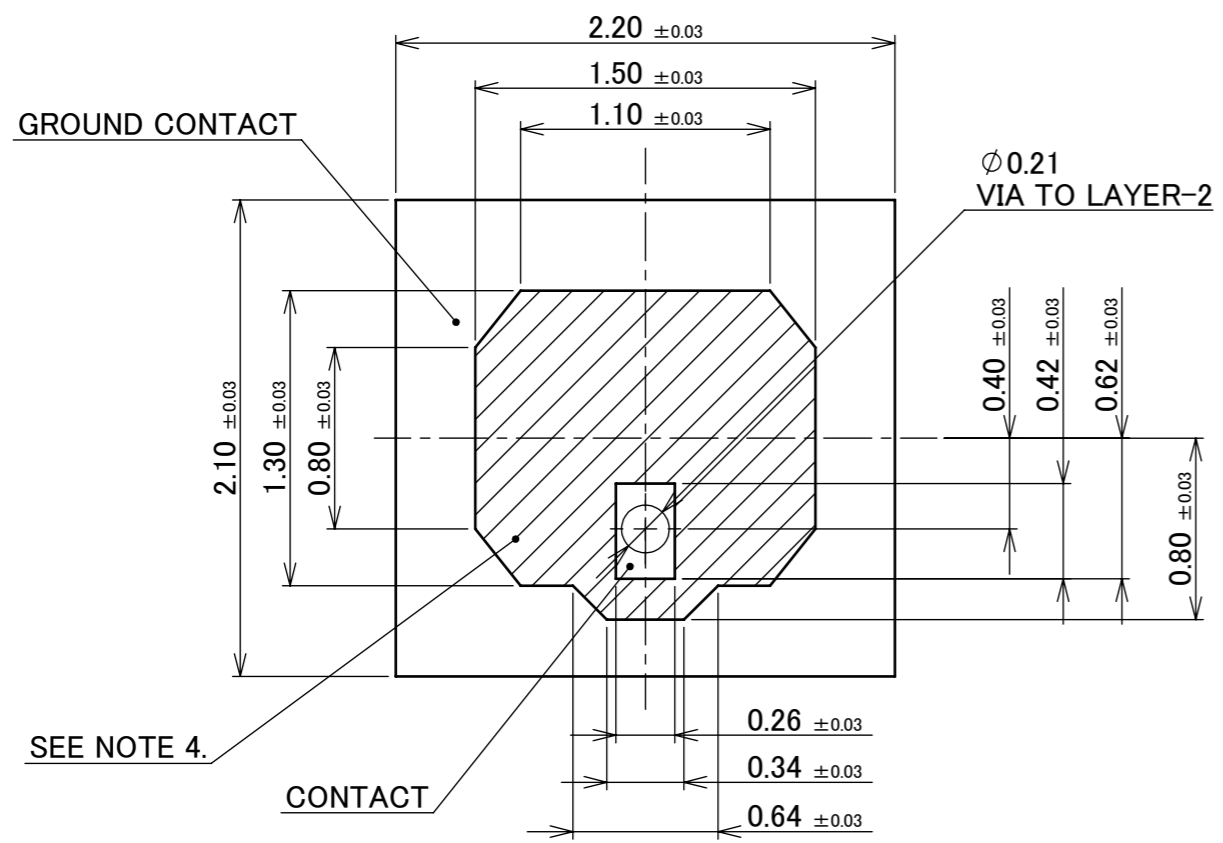
RECOMMENDED FOOTPRINT PATTERN
