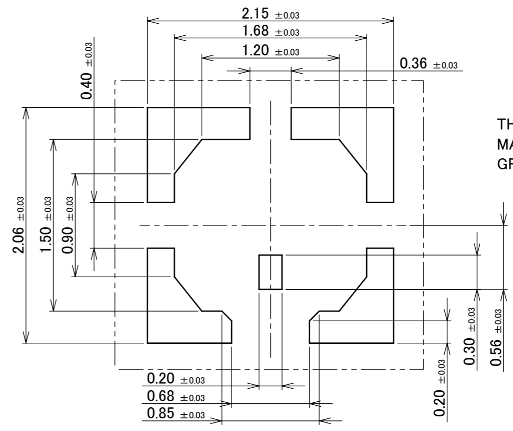
METAL MASK
