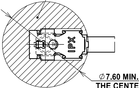
MATING AND LOCK CONDITION WITH MHF 4L LK HARNESS
