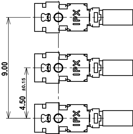
MHF 4L LK HARNESS UNLOCK CONDITION NARROW PITCH DIMENSIONS
