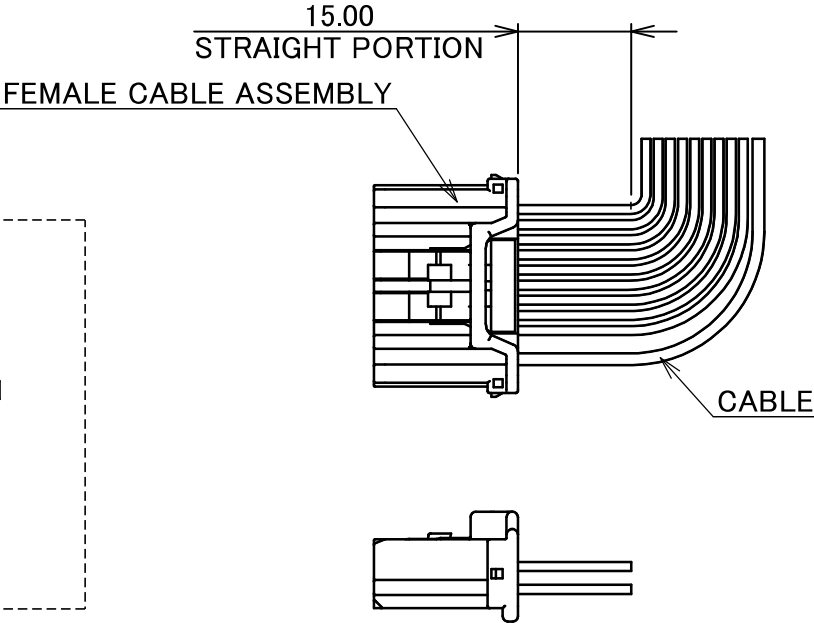
FEMALE CONNECTOR
