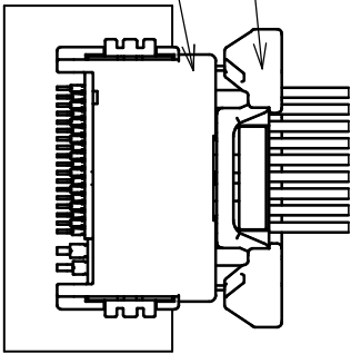
MALE ASSEMBLY
