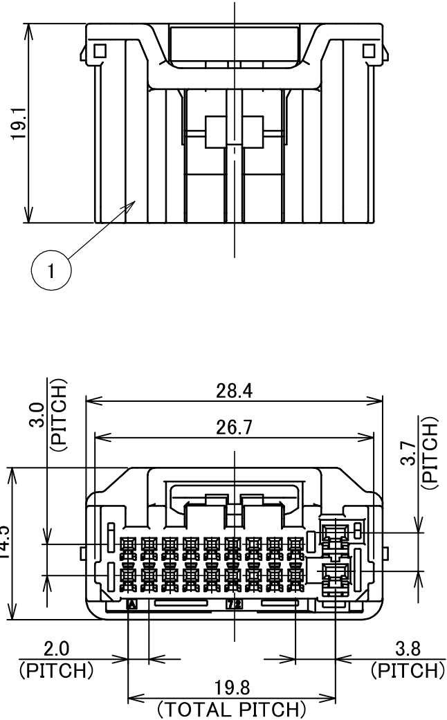
CODING - A PART NO.: V0124-020B-01/V0124-020B-02
