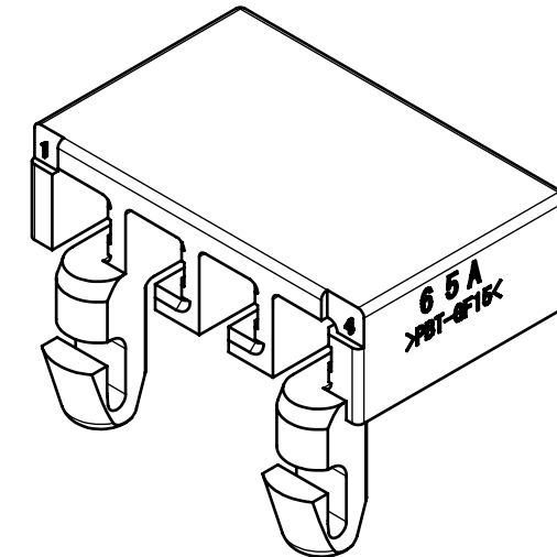
IARPB CONNECTOR 4P HOUSING PARTS NO. V0125-91004-01
