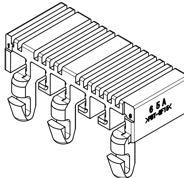
IARPB CONNECTOR 6P HOUSING PARTS NO. V0125-91006-01
