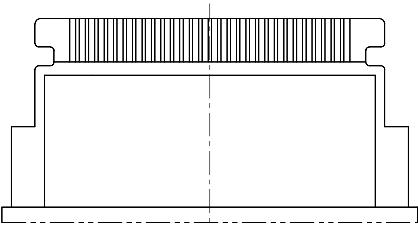
DETAIL Q 30P, 50P (S=5/1)
