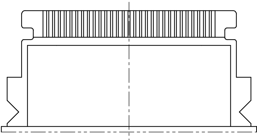
DETAIL P 30P, 50P (S=5/1)
