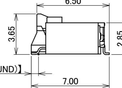
SECT. LL-LL (S=10/1)
