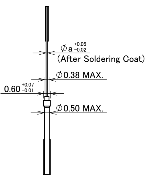
MICRO-COAXIAL CABLE DIMENSION
