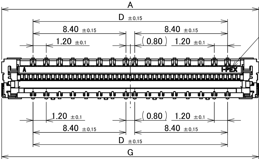
TOP VIEW
