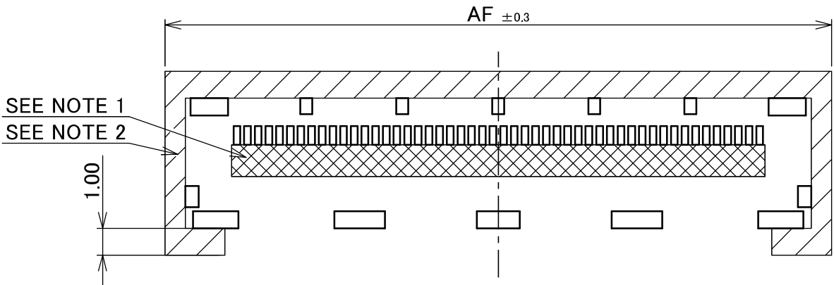
02TYPE 50P RECOMMENDED PCB LAYOUT [TYPE C] (S = 5 : 1)
