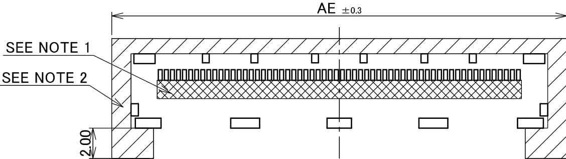
02 TYPE 60P RECOMMENDED PCB LAYOUT (S = 4 : 1)
