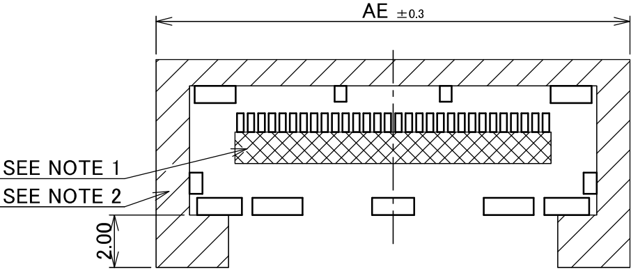
02 TYPE 30P RECOMMENDED PCB LAYOUT【TYPE B】 (S = 5 : 1)
