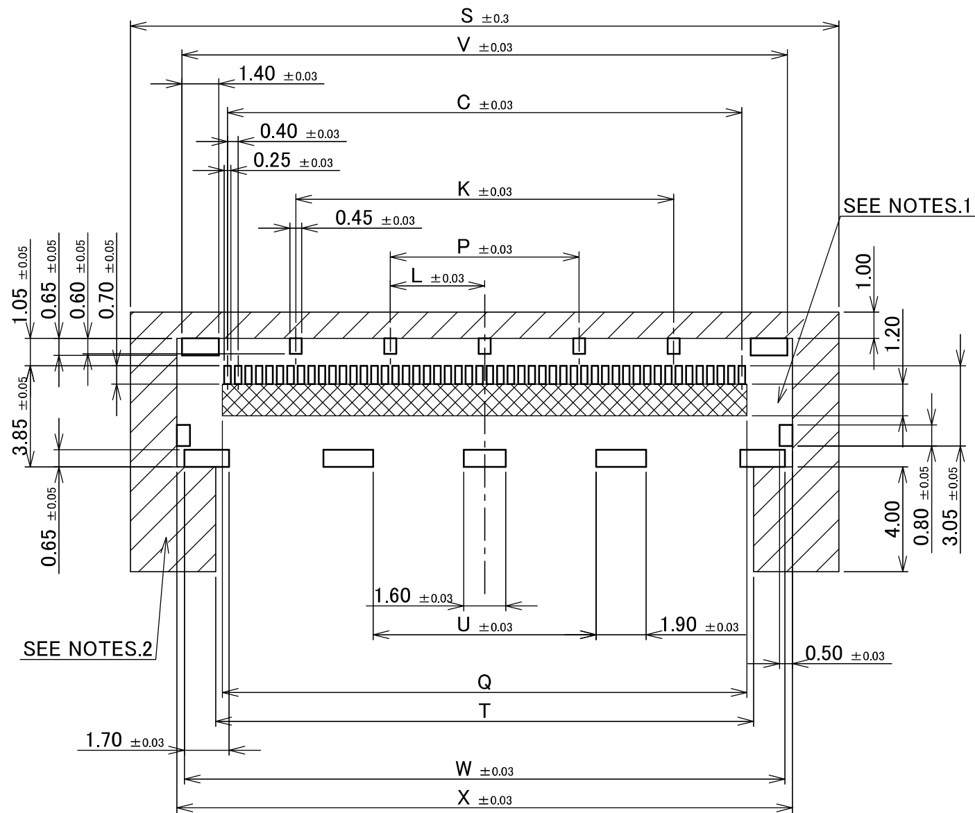
02TYPE 50P RECOMMENDED PCB LAYOUT [TYPE A] (S = 5 : 1)
