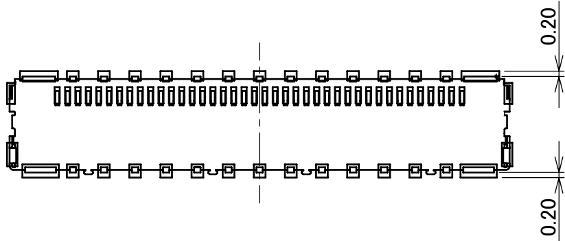
CONNECTOR ON RECOMMENDED FOOTPRINT PATTERN X01 TYPE
