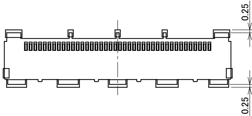
CONNECTOR ON RECOMMENDED FOOTPRINT PATTERN X02 TYPE
