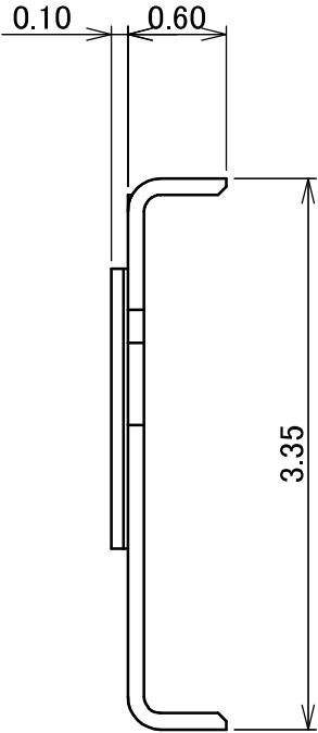
DETAIL X (S=20 : 1)
