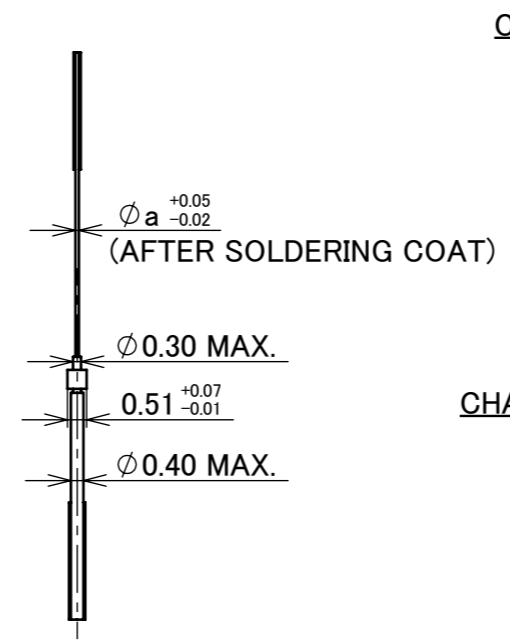
MICRO-COAXIAL CABLE AWG#**
