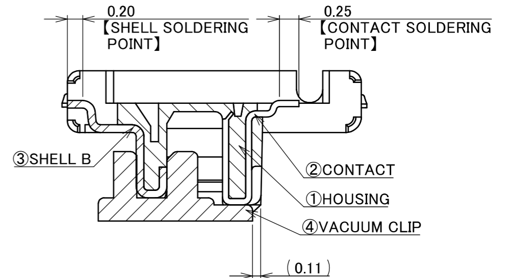
SECT. BB-BB (S=20 : 1)
