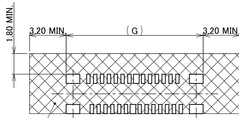
PATTERN A : WHEN USING A DOUBLE-SIDE REMOVAL JIG
