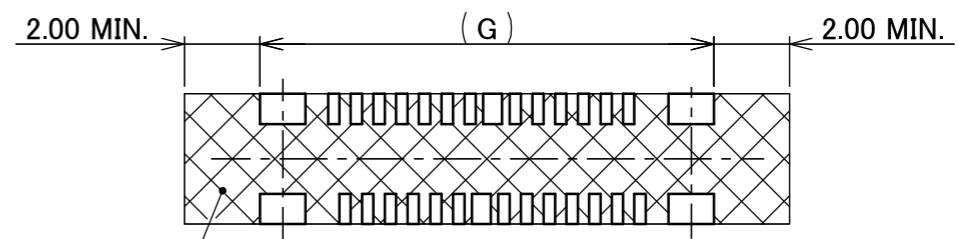
COMPONENT MOUNTING PROHIBITION AREA PATTERN B
