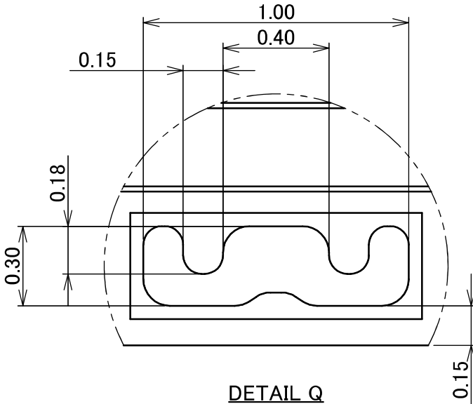
DETAIL Q (S= 50/1)
