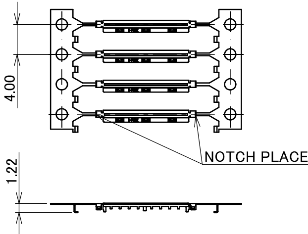
WITH CARRIER (S= 2/1)
