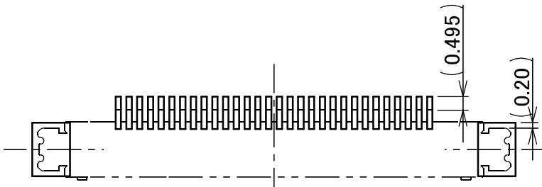
CONNECTOR ON RECOMMENDED FOOTPRIT PATTERN
