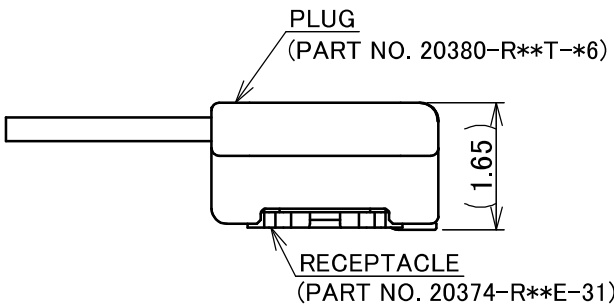
MATING CONDITION
