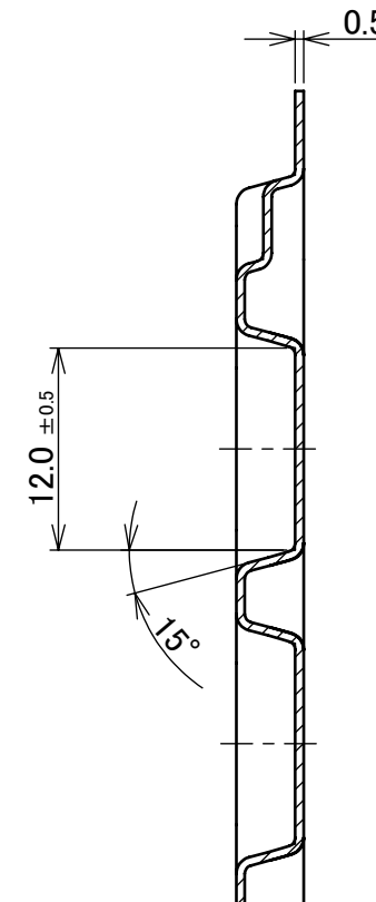
SECT. X-X (S=2/1)
