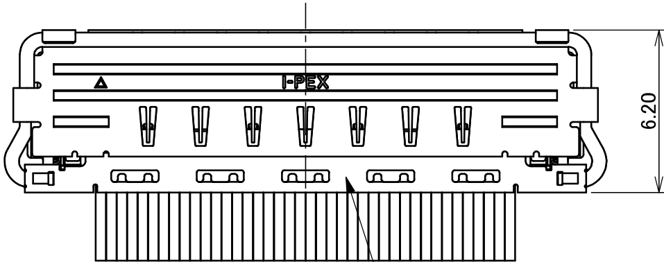
MATING CONDITION
