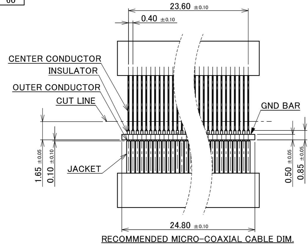
MICRO-COAXIAL CABLE AWG#**
