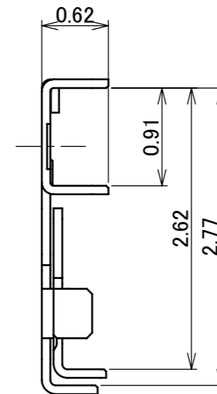
DETAIL AA (S=20/1)
