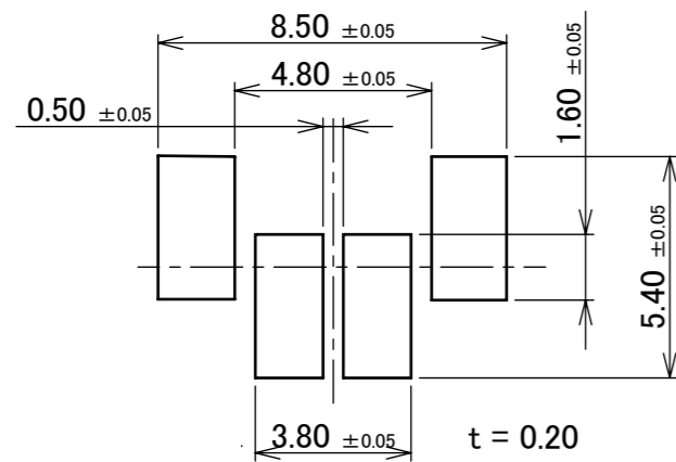
RECOMMENDED METAL MASK LAYOUT
