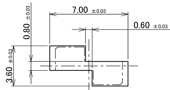
RECOMMENDED FOOTPRINT PATTERN
