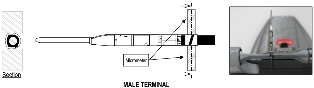
Fig 10. Insulation barrel crimp width measurement
