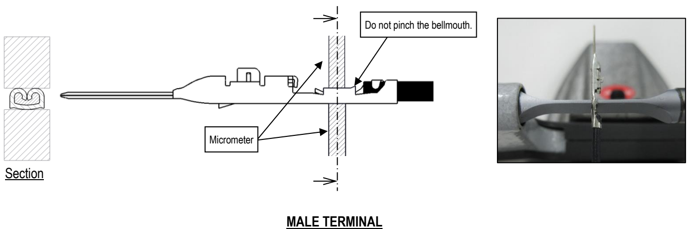
Fig 7. Wire barrel Crimp height measurement
