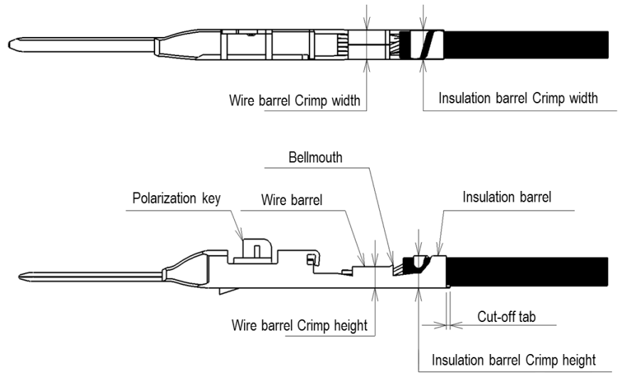
Fig.5 Male terminal part names
