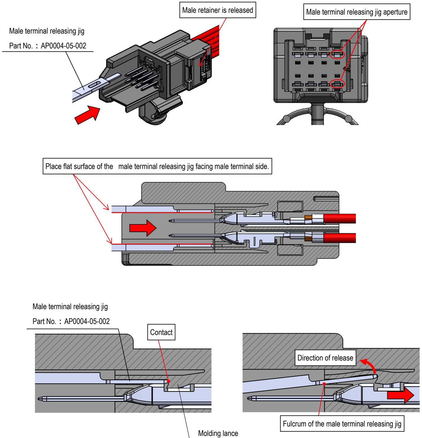
Fig.39 How to release the male terminal
