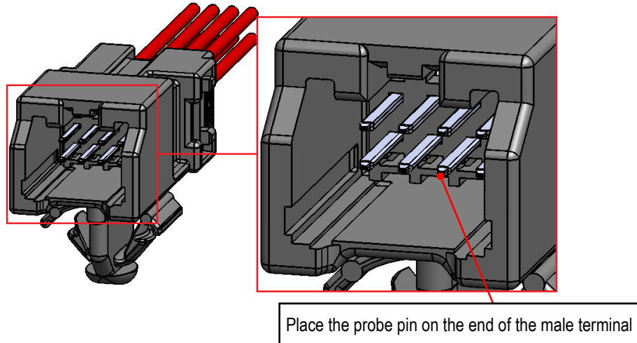
Fig.50 Conductivity test for male terminals (contacts)
