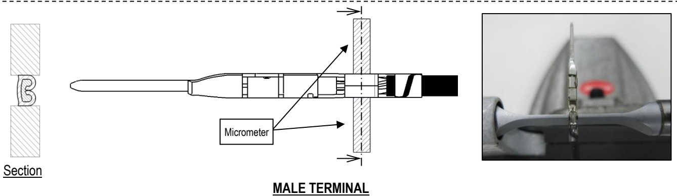
Fig 9. Wire barrel crimp width measurement
