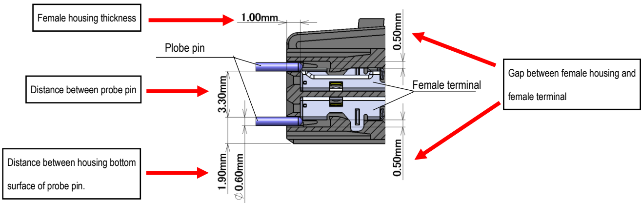
Fig.49 【Reference】Probe pin position on female connector
