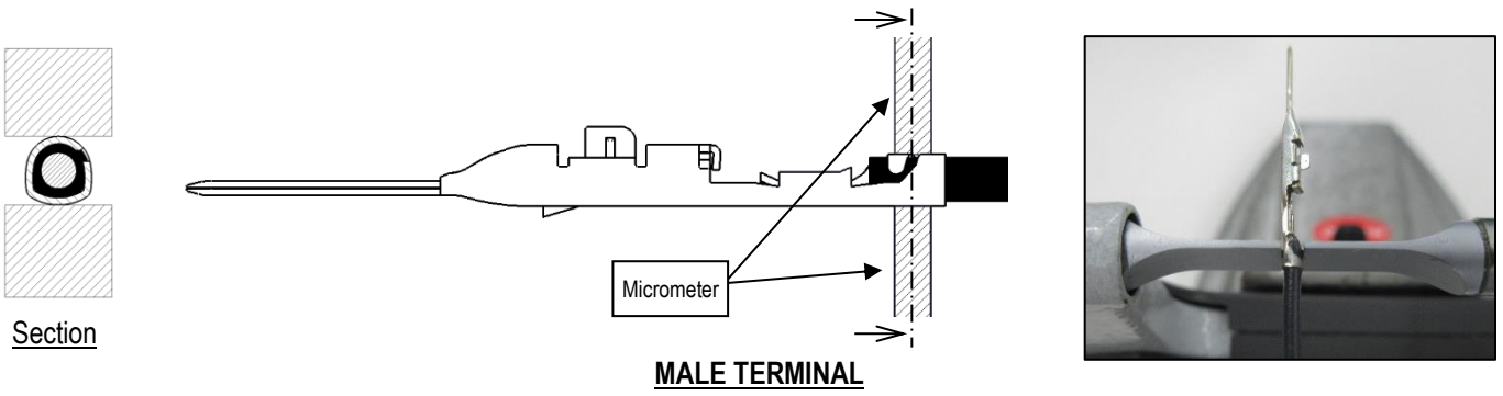
Fig 8. Insulation barrel Crimp height measurement
