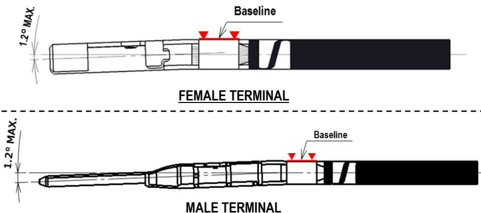
Fig.16 Twist terminal
