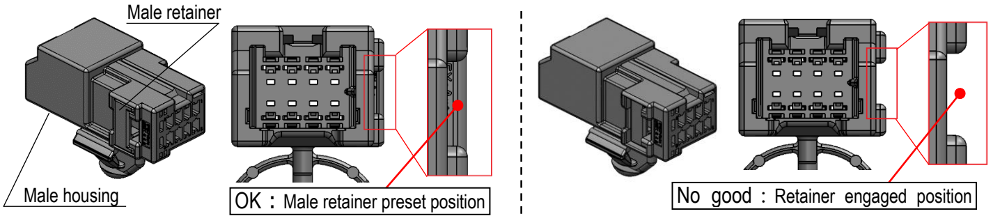
Fig.32 Checkpoint before engaging male retainer and the male housing.
