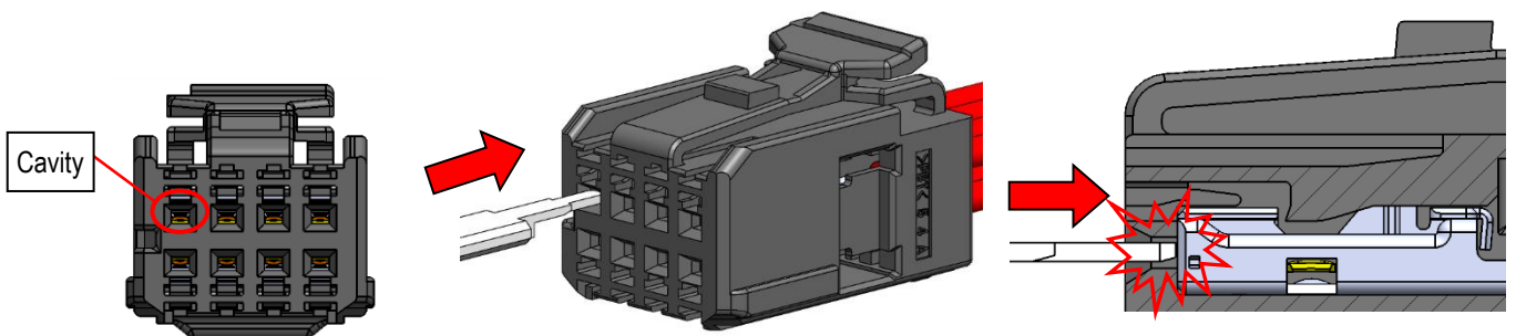
Fig. 43 Incorrect insertion of the terminal releasing jig
