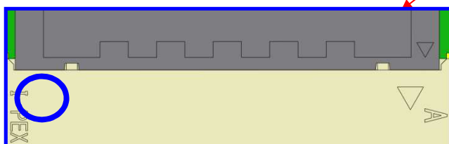
(a) 嵌合完了 / State of complete mating
