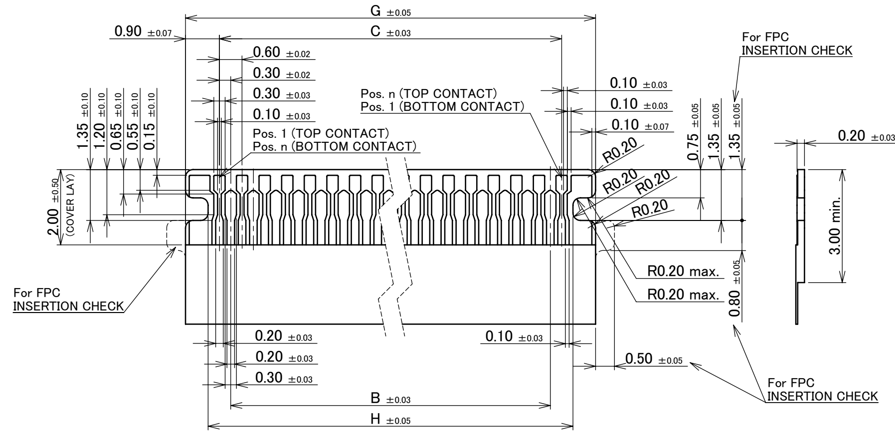
RECOMMENDED FPC LAYOUT
