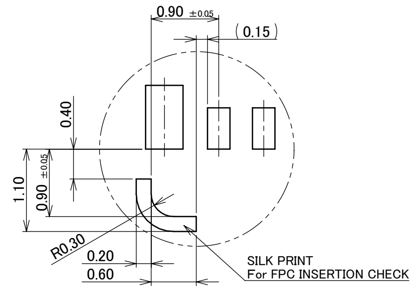
DETAIL AA (S=20/1)
