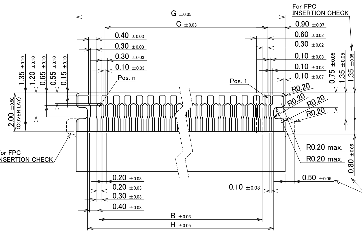
RECOMMENDED FPC LAYOUT (FOR BOTTOM CONTACT)
