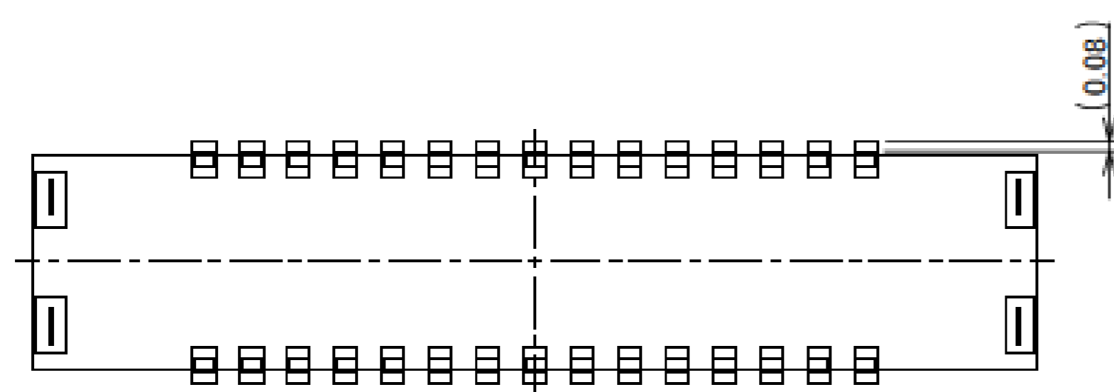
CONNECTOR ON RECOMMENDED FOOTPRINT PATTERN
