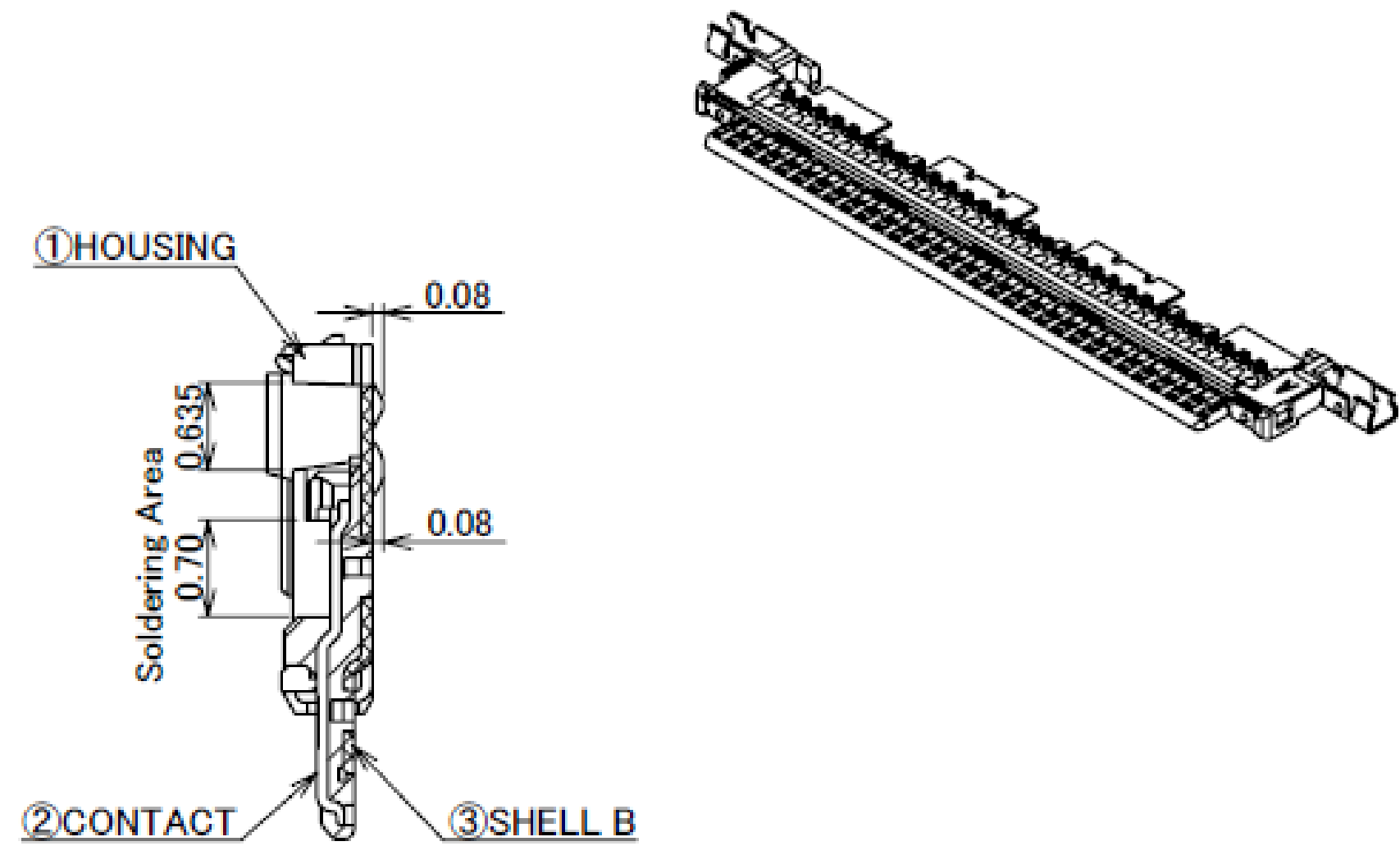
SECT. X-X (S=15/1)
